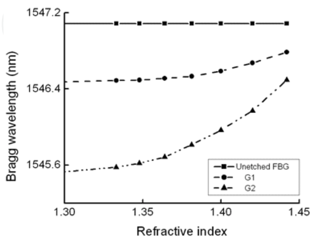
Figure 17. SRI sensitivity for un-etched, shallowly (G1) and deeply (G2) etched FBG in D-fibre.
