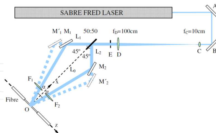
Figure 5. Two-beam holographic FBG inscription system.
