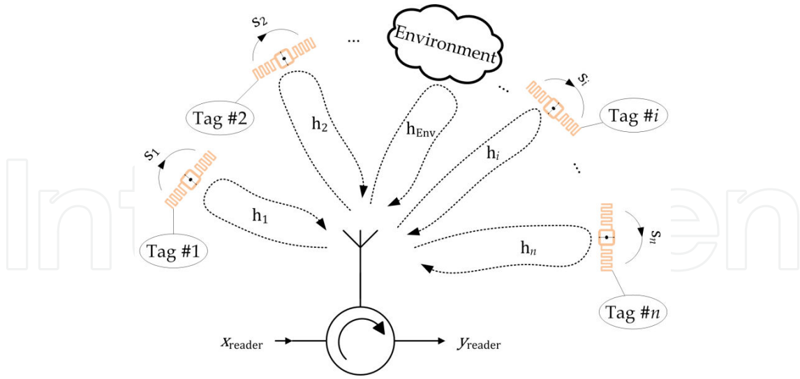
Figure 5. Scenario with passive RFID tags and reader in monostatic antenna setup
