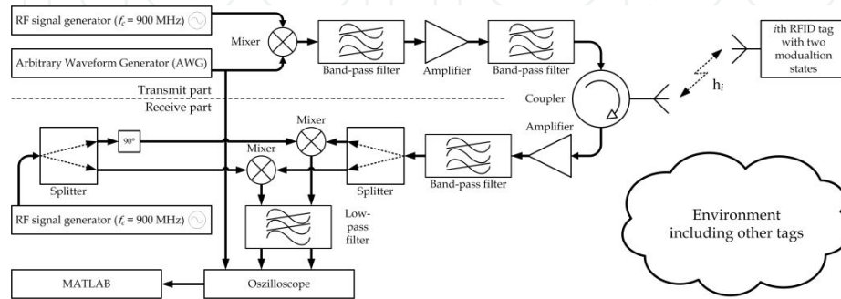
Figure 6. Experimental hardware architecture of the realized RFID localization system based on passive UHF RFID tags
