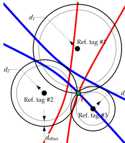
Figure 2. Example of hyperbolic trilateration using RFID tags as reference points
