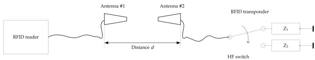
Figure 8. Measurement setup of RFID localization system
