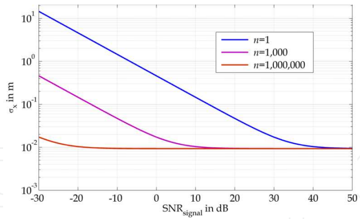
Figure 7. Cramér-Rao Lower Bound of the localization system
