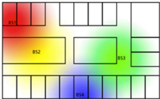
Figure 4. Electrical field strength distribution within a building to be used for WLAN positioning [20]
