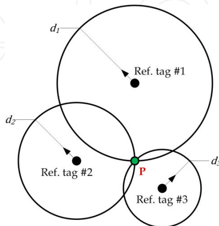
Figure 1. Example of trilateration with RFID reference tags
