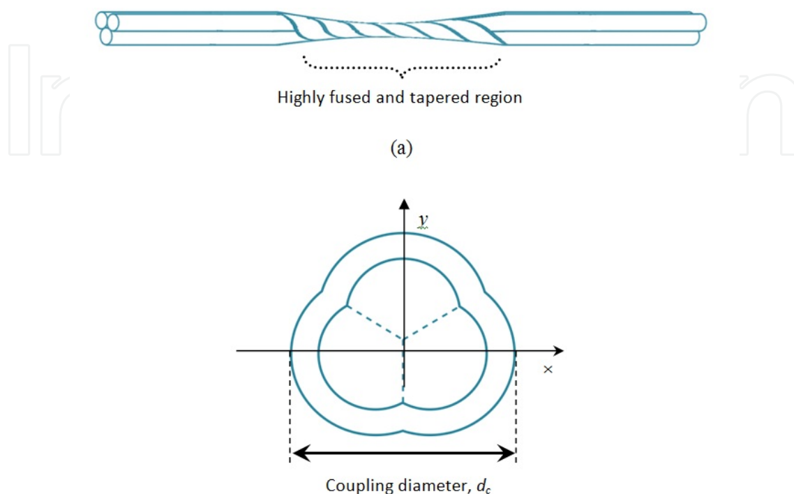
Figure 6. New schematic design of (a) highly-fused taper structure in the center of fiber bundle and (b) cross-section of fused region in fused 3 \times 3 biconical coupler
