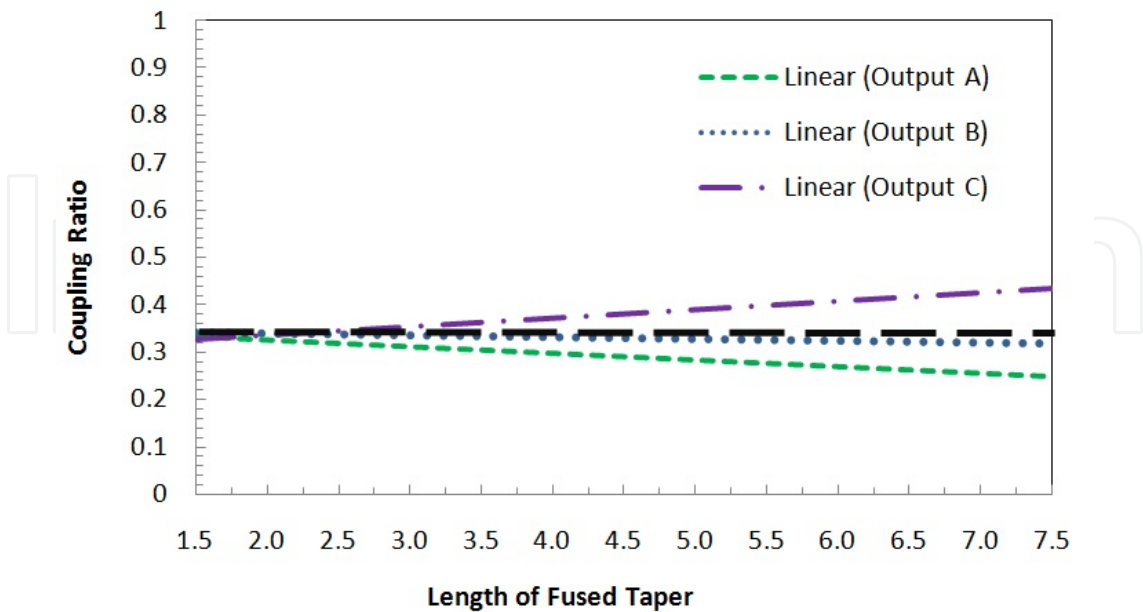
Figure 8. The coupling ratio of 3 \times 3 coupler with range of tapered length vary from 1.5 cm to 7.5 cm; the coupler has good coupling ratio ( \sim 0.33 ) for each port within the range of 3 cm to 1.5 cm
