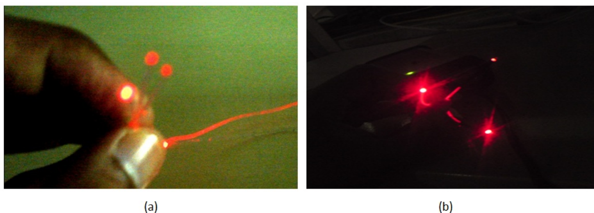
Figure 10. The results of experimental optical injection with 650\text{ nm} light source; (a) for the first generation of splitter and (b) for the second generation of LFT™ splitter.
