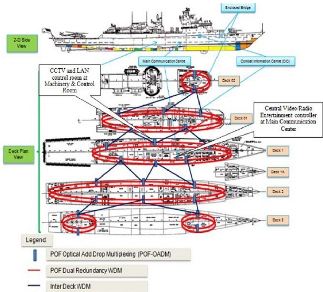
Figure 3. Deck-by-deck dual redundant POF-WDM backbone architectural network
