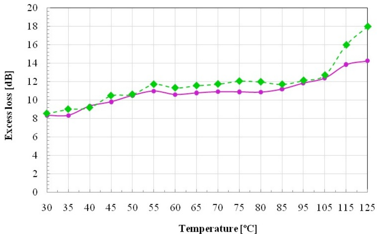
Figure 14. Excess loss variations as function of temperature for the splitter in bidirectional power injection
