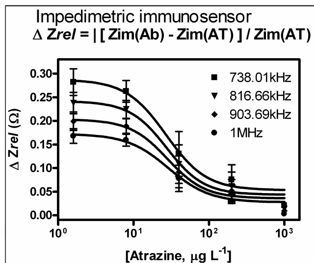
Figure 7. Impedimetric immunosensor responses using the relative difference of Zim at high frequencies from 738.01 kHz to 1 MHz. Reprinted from Sensors and Actuators B , 129/2, Ángel Rodríguez, Enrique Valera, Javier Ramón-Azcón, F.-J. Sanchez, M.-P. Marco, Luis M. Castañer, Single frequency impedimetric immunosensor for atrazine detection, 921-928, Copyright (2008), with permission from Elsevier.
