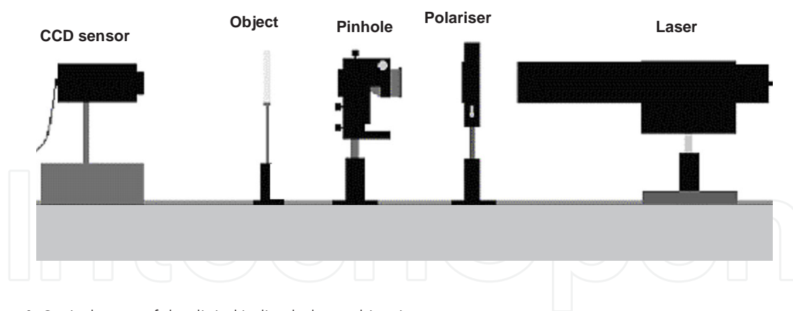
Figure 1. Optical setup of the digital in-line holographic microscope
