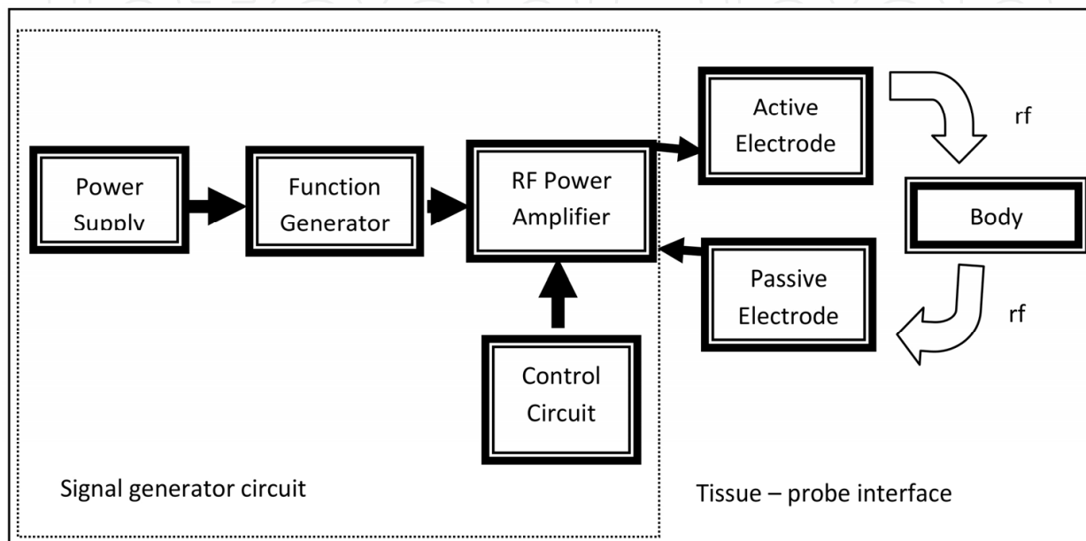
Figure 1. Block diagram of the RF ablation circuits
