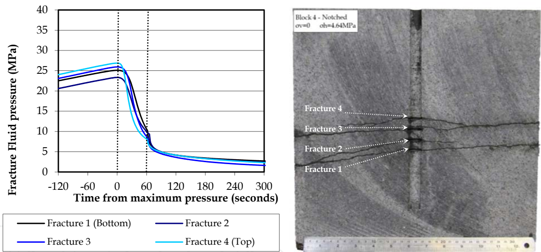
Figure 5. Fracture pressure records and 2-dimensional cross section of Block 4, after Bunger et al. [5].
