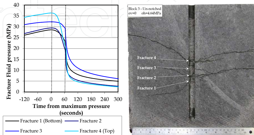
Figure 2. Fracture pressure records (the vertical dotted lines represent maximum pressure and shut in respectively) and 2-dimensional cross section of Block 3 (Hydraulic Fractures can be seen as dark grey cracks on the cross-section image), after Bunger et al. [5].
