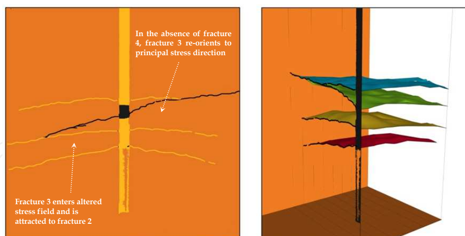
Figure 10. A 2-dimensional cross-section of Block 6 showing the deflected path of fracture three (left) and a 3-dimensional reconstruction of the fracture paths in Block 6 (a video animation of this fracture can be viewed at http://youtu.be/ZCMBWGI_8-Y ).
