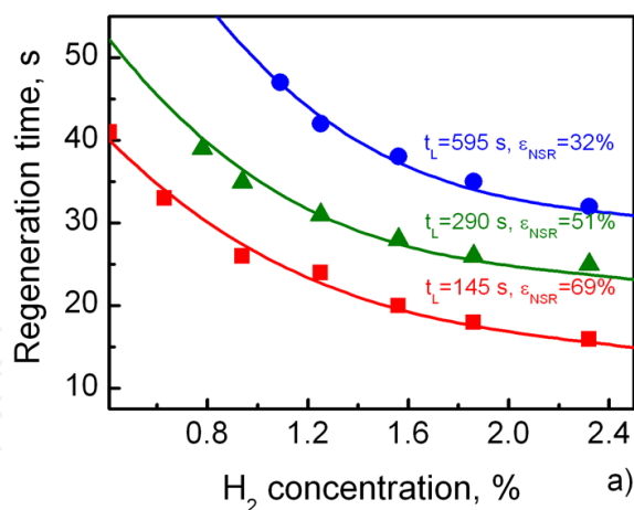
Figure 11. Operation map of the Pt-Ba/Al 2 O 3 monolithic catalyst. Relationship between operational variables ( C_{H_2} , t_P , t_R ) for carrying out the NSR process efficiently.
