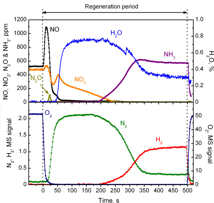
Figure 7. Evolution of NO, \text{NO}_2 , \text{N}_2\text{O} , \text{NH}_3 and \text{H}_2\text{O} concentrations by FTIR and MS signals of \text{O}_2 , \text{N}_2 and \text{H}_2 , during Pt-BaO/ \text{Al}_2\text{O}_3 catalyst regeneration at 330 °C.
