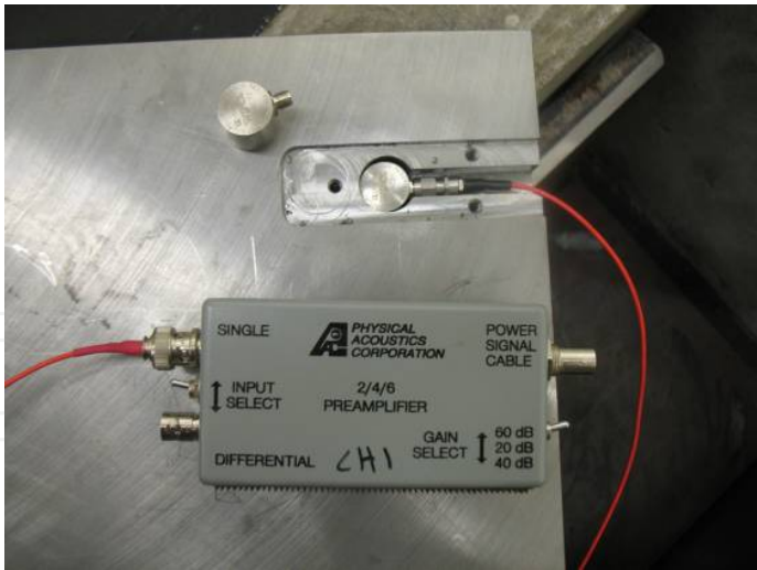
Figure 6. AE sensor installed in a loading platen.
