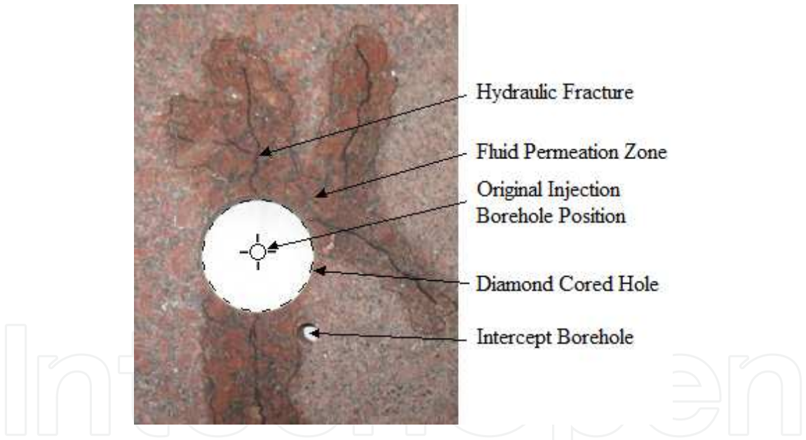
Figure 7. Cross-section from an unconfined granite hydraulic fracturing test.
