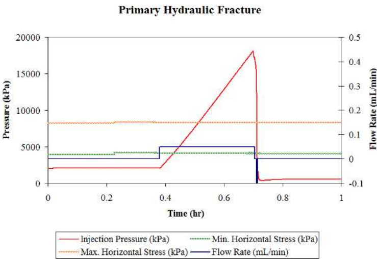
Figure 9. Hydraulic data plot for primary fracture.
