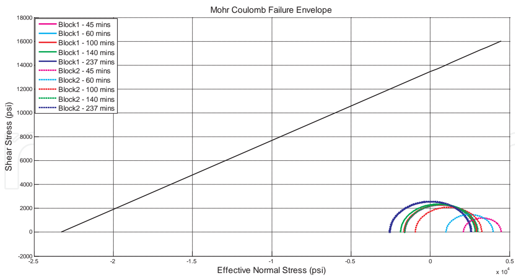
Figure 6. Mohr – Coulomb failure envelope for C_0 = 46570 \text{ psi} – Well A
