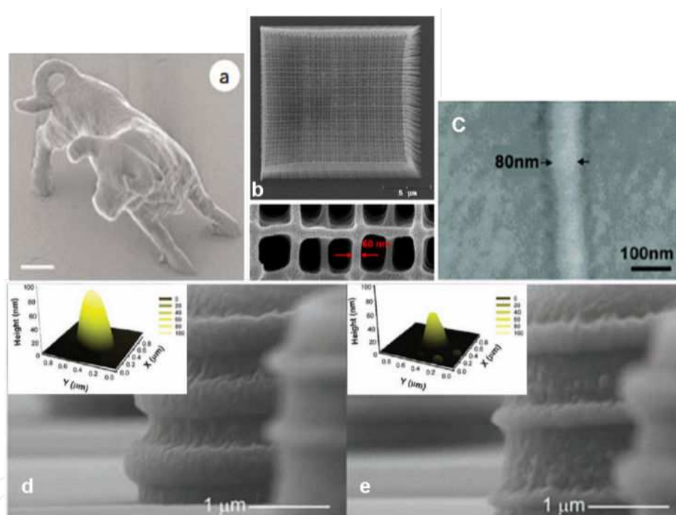
Figure 4. Improving spatial resolution of two-photon microfabrication by different strategies during the past decade. a) the famous microbull exhibiting 120 nm features size due to intrinsic properties of TPS ( \lambda = 780 nm, \lambda/6.5 ; Kawata et al. 2001), b) Photonic crystal with 60 nm features size due to the use of shorter wavelength ( \lambda = 532 nm, \lambda/8 ; Haske et al. 2007), c) 80 nm linewidth by using a high efficient photoinitiator ( \lambda = 800 nm, \lambda/10 ; Xing et al. 2007), d) and e) microtower fabricated by using a conventional TPS and a STED-like TPS, respectively. In d and e insets, AFM measurements of voxel size are shown. e) inset is the current smallest axial resolution (40 nm) for a voxel thanks to a STED-like method ( \lambda = 800 nm, \lambda/20 ; Li et al. 2009). Reproduced from the respective references.
