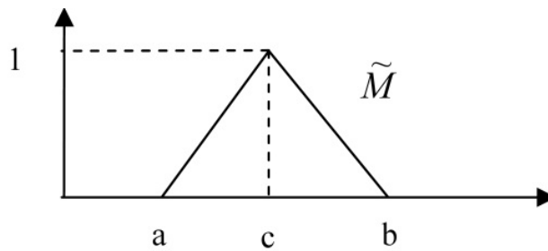
Figure 1. Triangular fuzzy number, \tilde{M} = T(a, c, b) .
