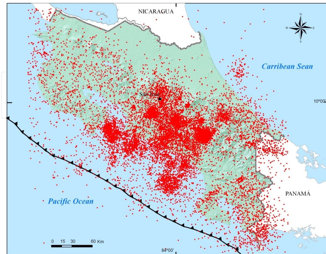
Figure 9. Background seismicity in Costa Rica from 1992 through 2009. Circles are earthquakes. Several clusters represent the most important seismic zones of Costa Rica. The sum of these clusters generates a zone of concentrated seismicity in Central Costa Rica. MAT: Middle American Trench.
