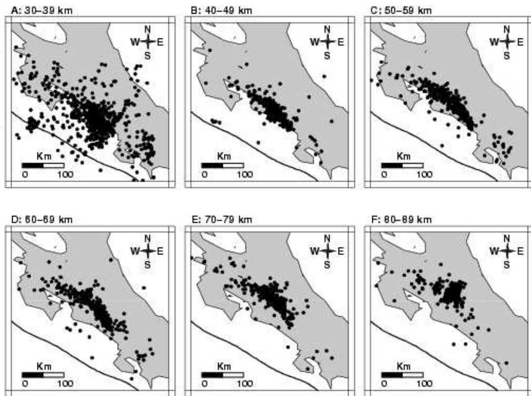
Figure 10. Cumulative numbers of located earthquakes, separated into six depth ranges, within or near the Costa Rican territory. These graphs plot earthquakes detected and located by the Red Sismologica Nacional (RSN: ICE-UCR) from 1992 to 2009. Depth ranges are in km.
