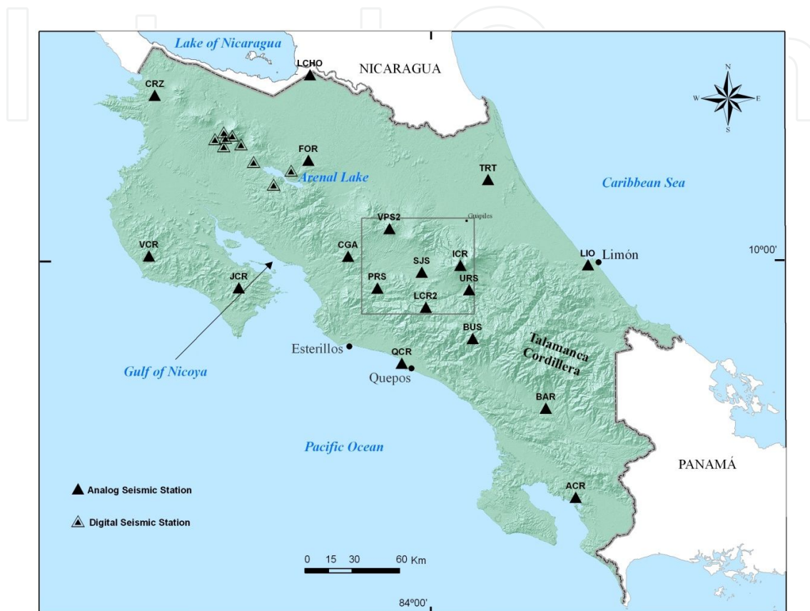
Figure 2. Seismic stations of the Red Sismologica Nacional (RSN: ICE_UCR) shown with triangles. Black triangles are analog stations. The digital stations are indicated by open triangles.
