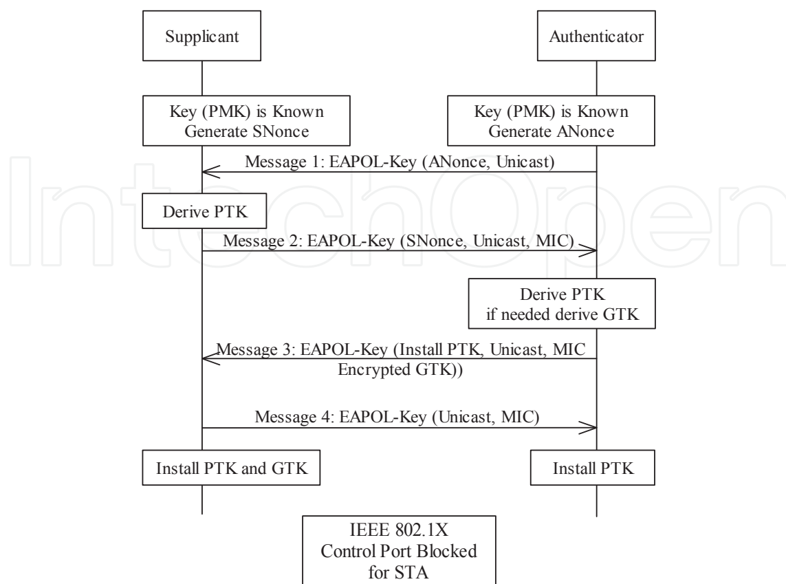
Figure 2. Establishing pairwise & group keys [6]
