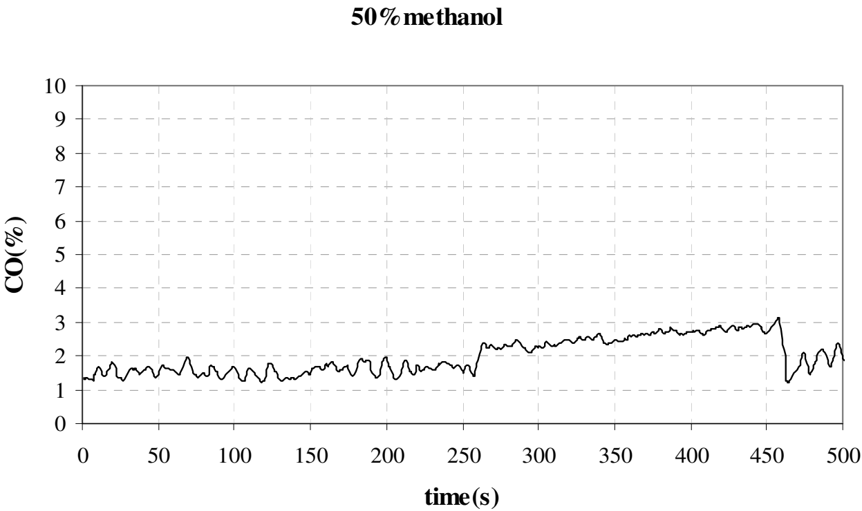
Figure 7. The CO variation when mixture of gasoline-50%methanol is used as fuel.
