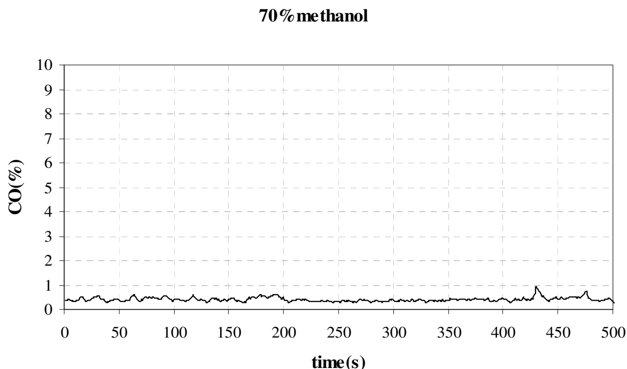
Figure 9. The CO variation when mixture of gasoline-70%methanol is used as fuel.
