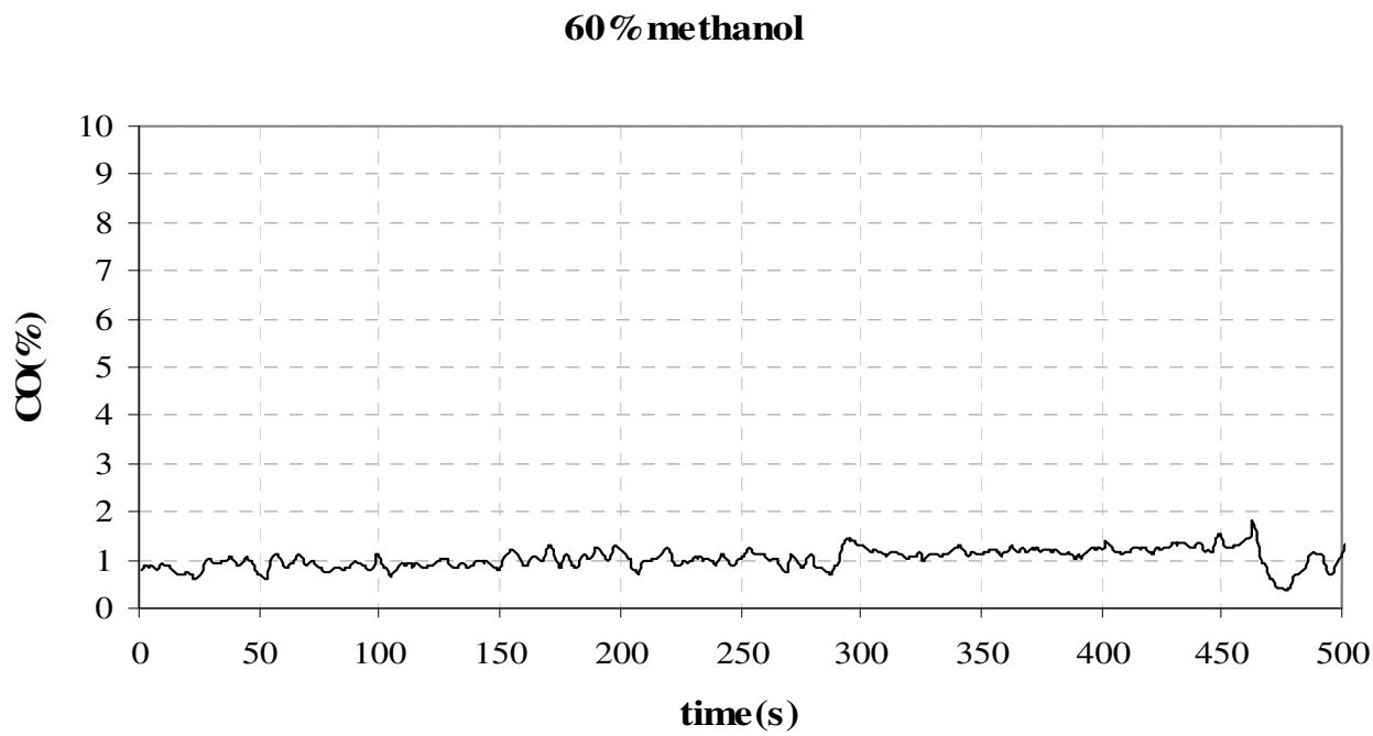
Figure 8. The CO variation when mixture of gasoline-60%methanol is used as fuel
