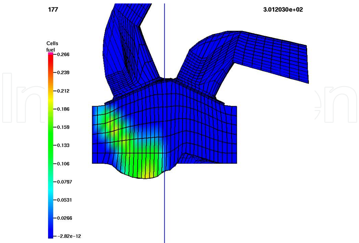
Figure 21. Participation of the gaseous phase in combustion chamber in stratified charge mode at 2400 rpm at 60° before TDC (Top Death Center)
