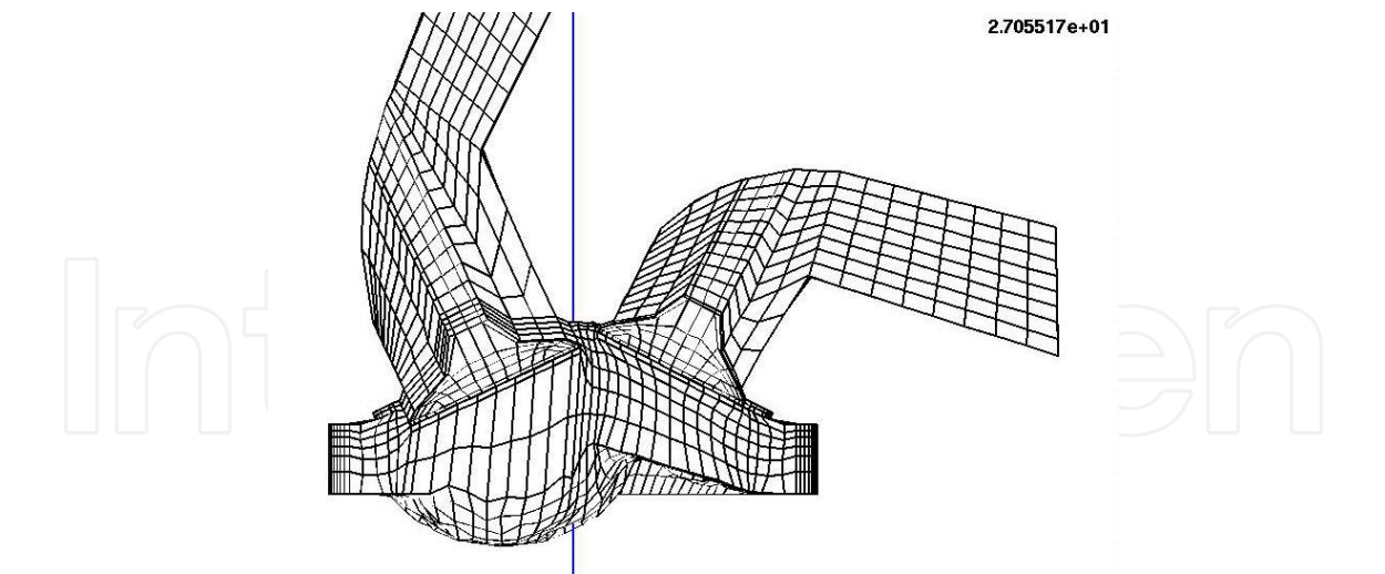
Figure 20. Engine mesh at 27 deg ATDC
