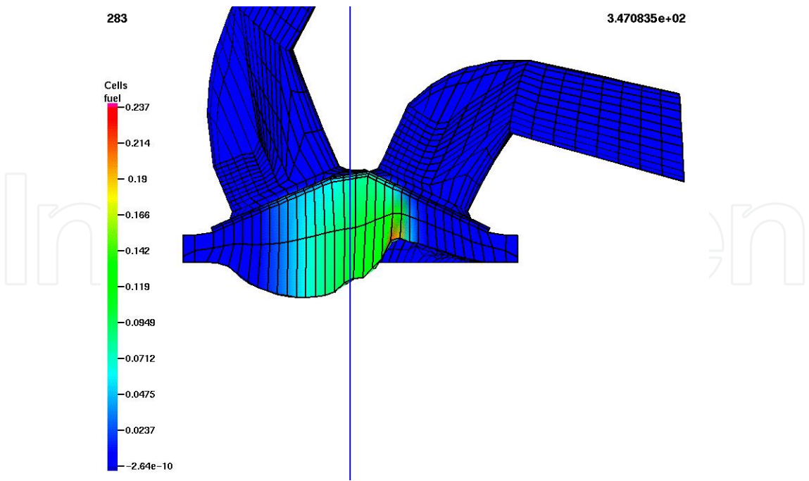
Figure 22. Participation of the gaseous phase in combustion chamber in stratified charge mode at 2400 rpm at 11° before TDC
