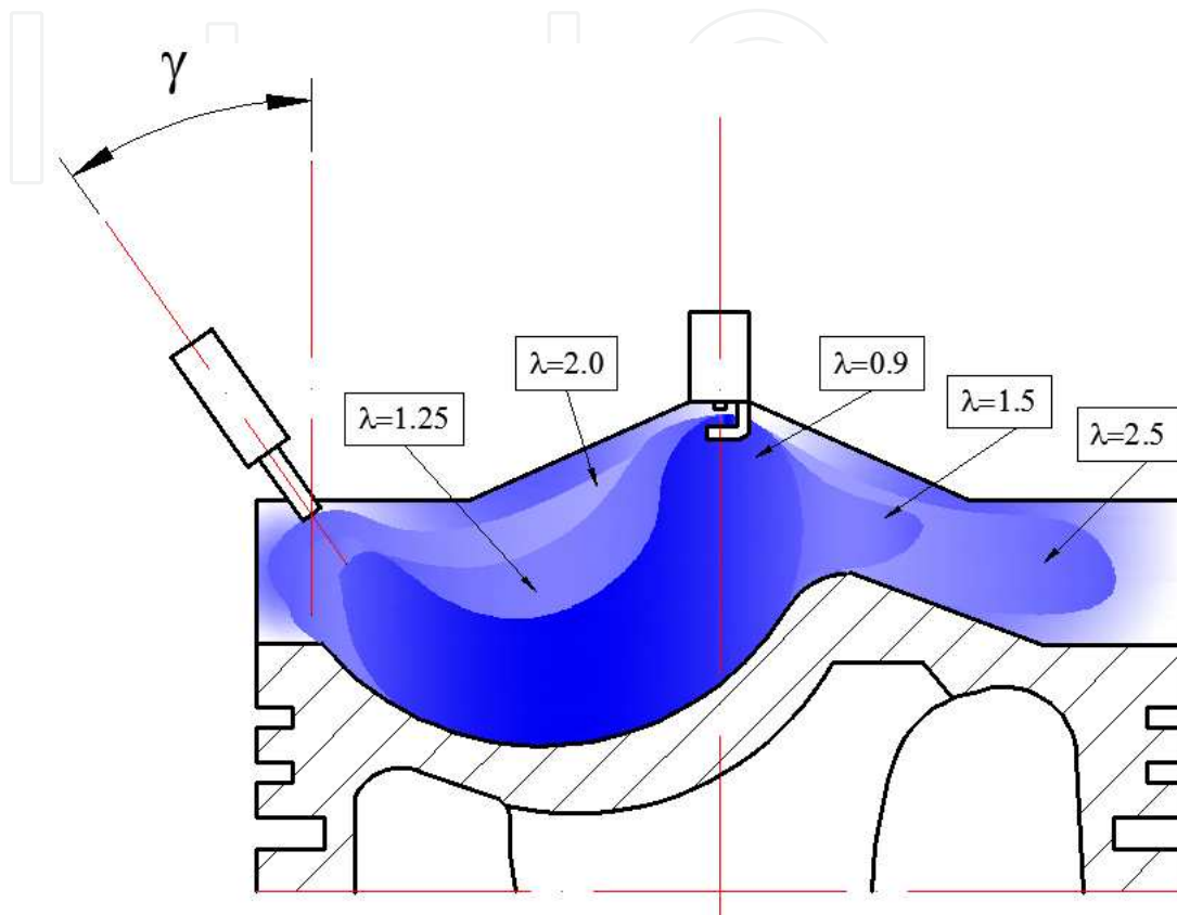
Figure 1. Variation of fuel mixture in combustion chamber.
