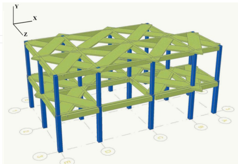
Figure 4. Rigid diaphragms in 3D RB framed building
