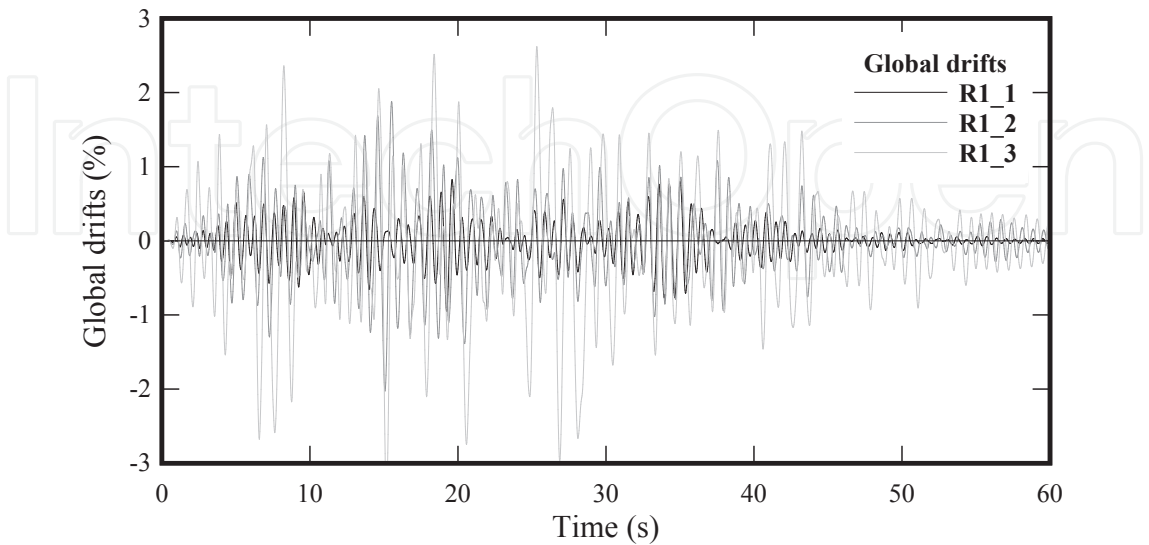
Figure 7. Global drifts. R1 earthquake. Frame C. OB building.
