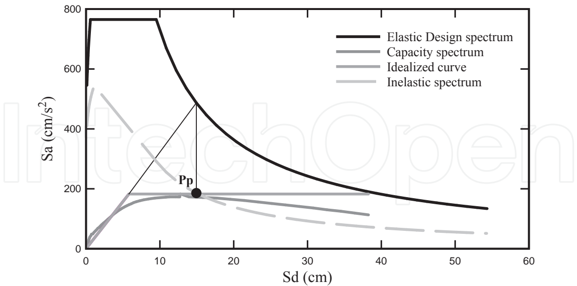
Figure 6. Performance point of Frame C. OB Building, determined by N2 procedure
