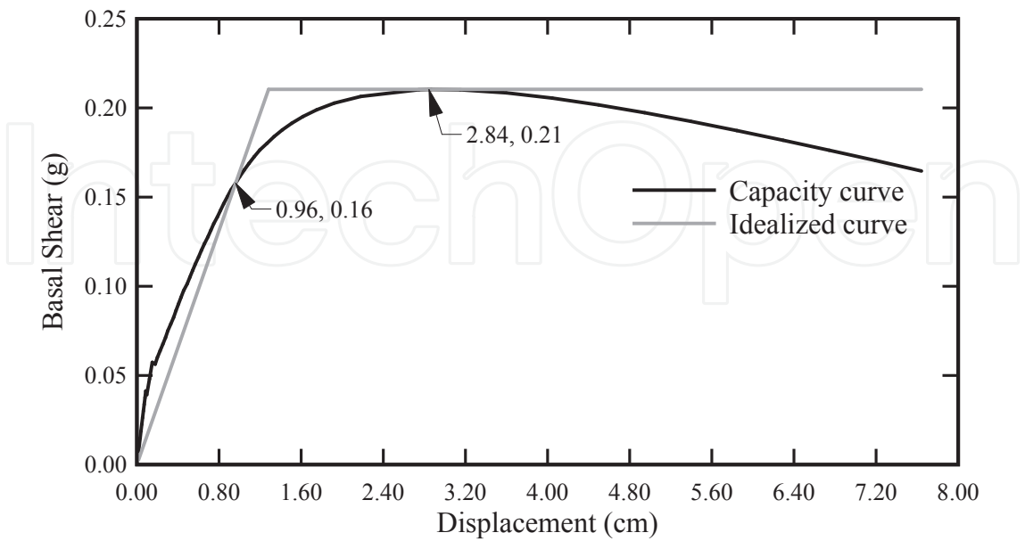
Figure 5. Normalized and idealized capacity curves. Frame C. OB building
