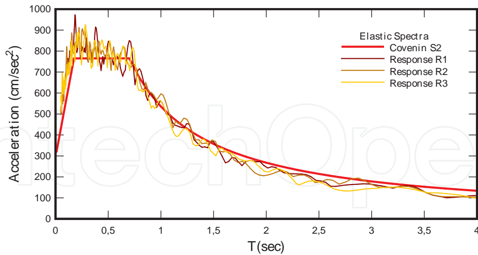
Figure 3. Elastic response spectra from elastic design spectrum-compatible accelerograms
