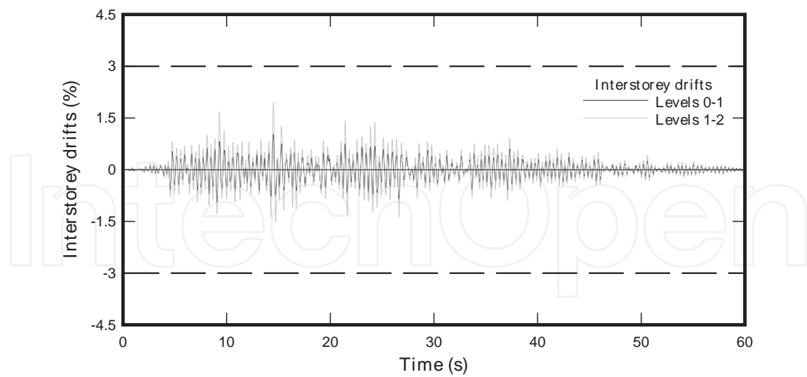
Figure 12. Interstorey drifts. R1_3 earthquake. Frame C. DBDB building
