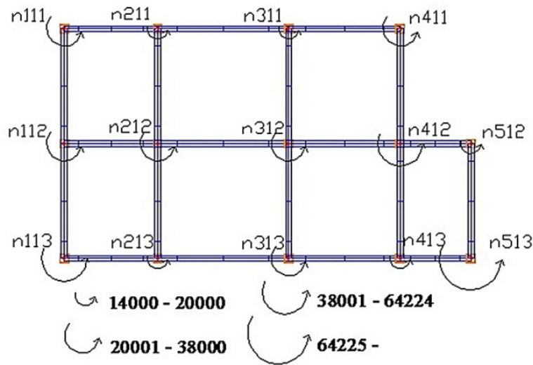
Figure 14. Torsional moments for earthquake 100% (X). Plant detail.
