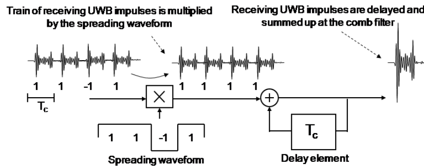
Figure 25. Comb filter principle in the receiver.
