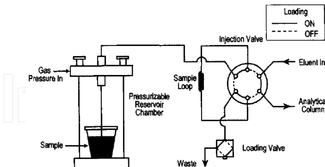
Figure 8. IC system configuration for direct-injection sample loading [21].
