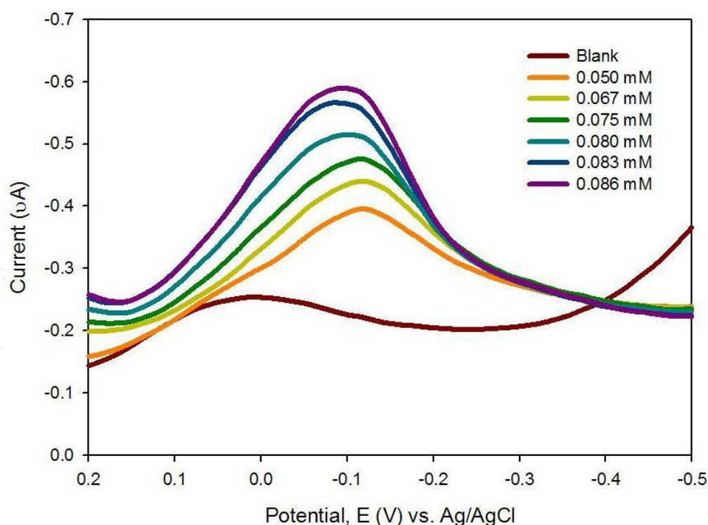
Figure 3. Net cathodic differential pulse voltammograms (DPVs) of the Pt/PANI/HRP biosensor in the presence of increasing concentrations of \text{H}_2\text{O}_2 as substrate. The experimental conditions were: frequency, 20 Hz; amplitude, 20 mV; and potential step, 20 mV.
