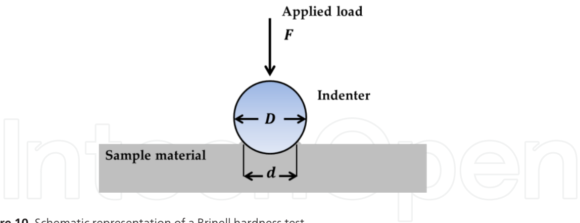
Figure 10. Schematic representation of a Brinell hardness test
