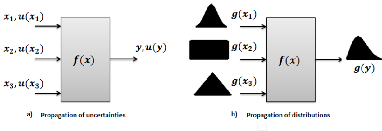
Figure 1. Illustrations of the methodologies of a) propagation of uncertainties, where x_1, x_2 and x_3 are input quantities, u(x_1), u(x_2) and u(x_3) are their respective uncertainties and y and u(y) are the measurand and its uncertainty, respectively; and b) propagation of distributions, where g(x_1), g(x_2) and g(x_3) are the distribution functions of the input quantities and g(y) is the distribution function of the measurand
