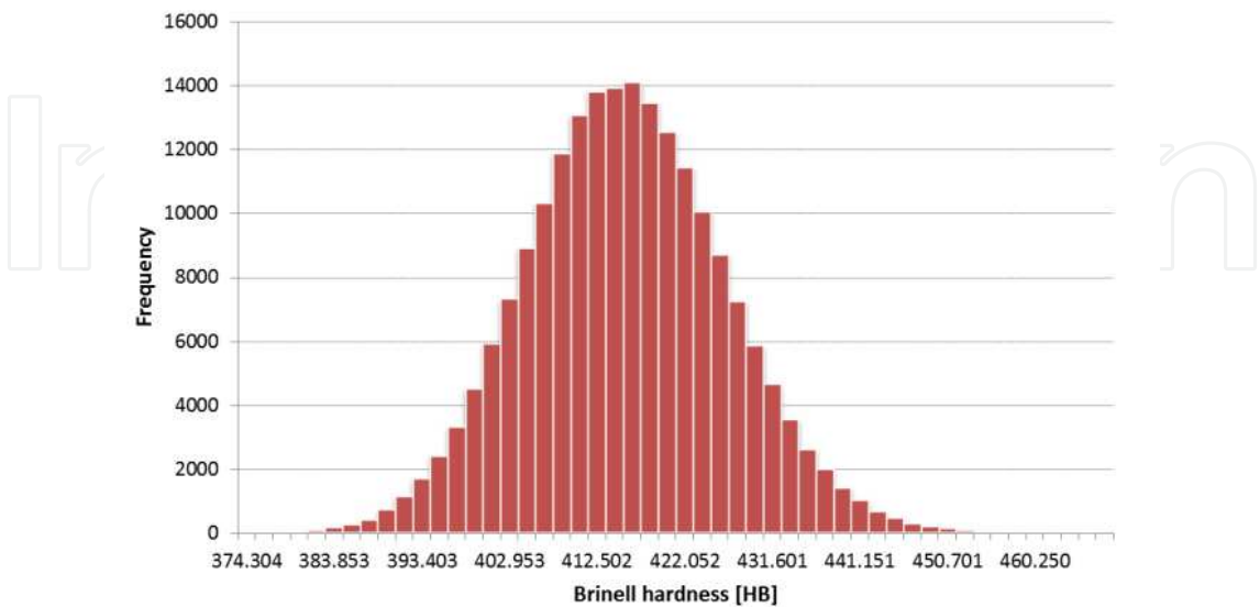
Figure 12. Histogram representing the resulting PDF for the Brinell hardness estimated by Monte Carlo simulation
