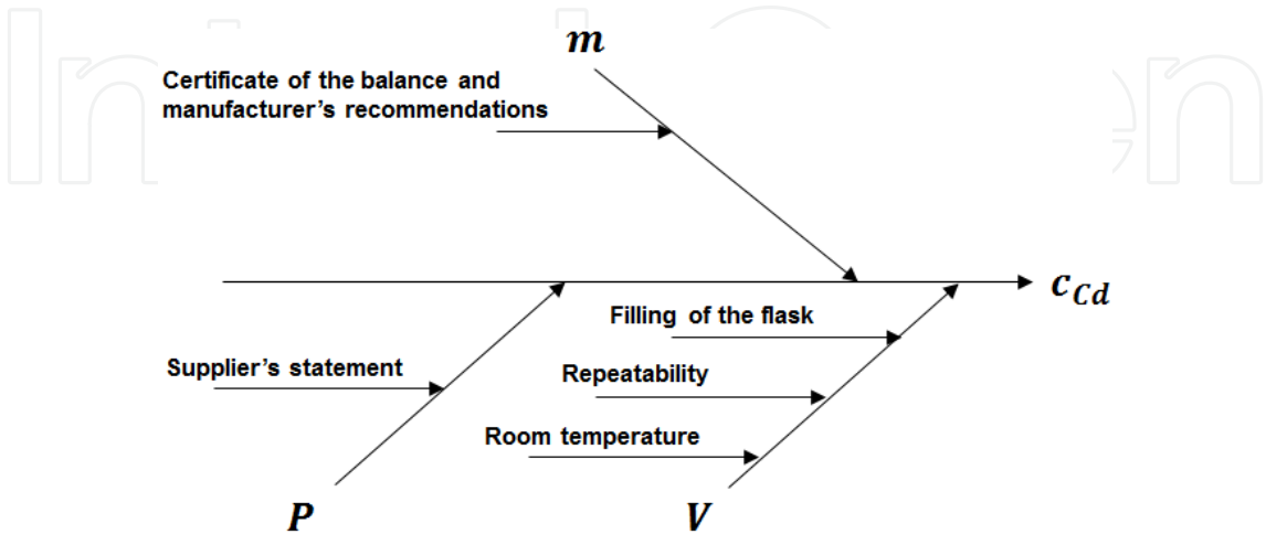
Figure 8. Cause-effect diagram for the preparation of a standard cadmium solution
