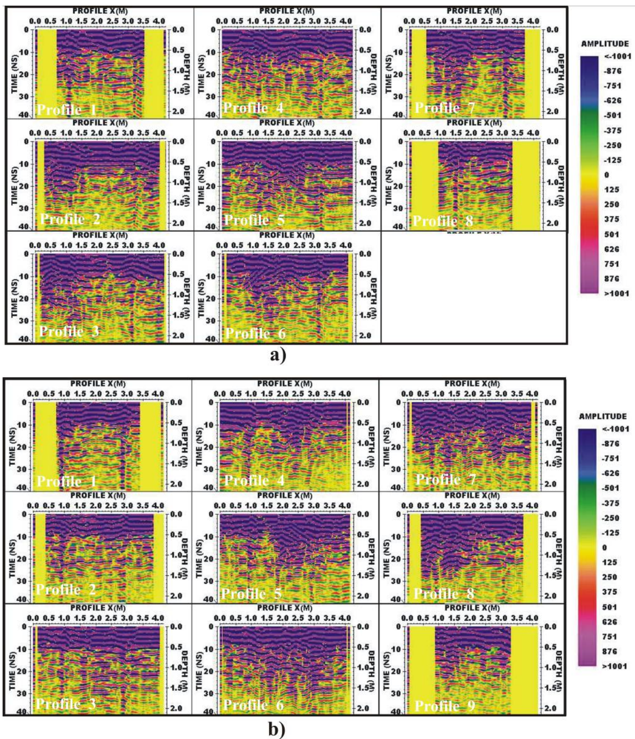
Figure 19. Processed radargrams of the profiles along (a) the east-west direction and (b) the south-north direction inside the Zeynel Bey tomb.
