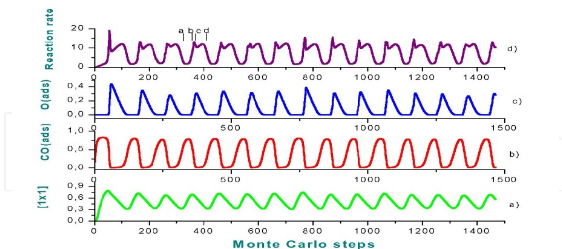
Figure 1. Self-oscillations of the model variables at M = 100 and N = 500 . a) Coverage *_{1 \times 1} = *_{1 \times 1} + CO_{ads}^{1 \times 1} + O_{ads}^{1 \times 1} , b) CO_{ads} = CO_{ads}^{1 \times 1} + CO_{ads}^{hex} , c) O_{ads}^{1 \times 1} , d) specific reaction rate. Parameter values: k_1 = 2.94 \times 10^5 ML/s Torr, P_{CO} = 5 \times 10^{-5} Torr, k_2 = 4 s ^{-1} , k_3 = 0.03 s ^{-1} , k_4 = 3 s ^{-1} , k_5 = 2 s ^{-1} , k_6 = 5.6 \times 10^5 ML/s Torr, P_{O_2} = 10^{-4} Torr, [26, Table 1].
