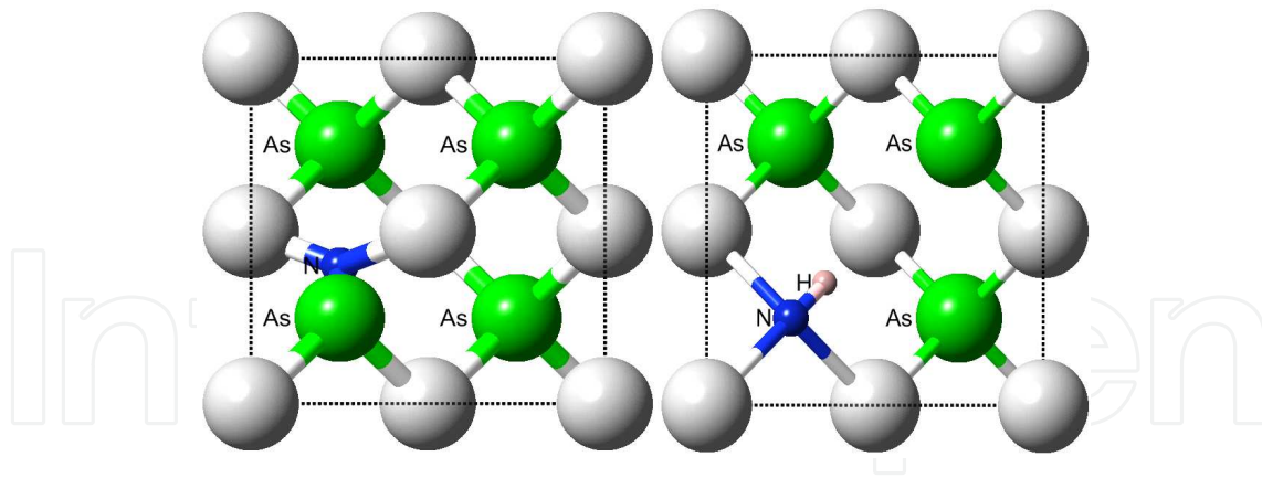
Figure 18. The split interstitial (N-As)_{As} (left) and N-H-V_{Ga} (right) as a possible origins of E1 and H2, respectively.
