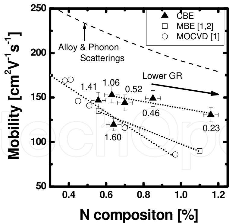
Figure 7. Hole mobility at room temperature in p-GaAsN films grown by CBE, MBE, and MOCVD as a function of N composition. The mobility is the value at room temperature. The dashed line represents the estimated mobility limited by the alloy and phonon scatterings. In the case of CBE, the growth rate (GR) is shown in the unit of \mu\text{m/h} . The dotted lines are a guide for the eye.
