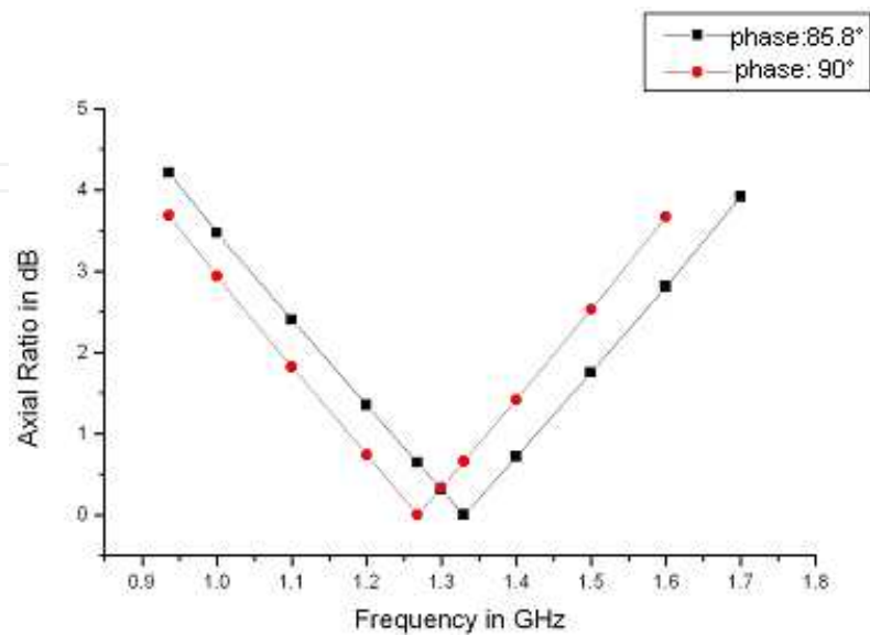
Figure 10. Axial ratio bandwidth of phase excitation has an offset at the central frequency in case of E1/E2=0\text{dB}
