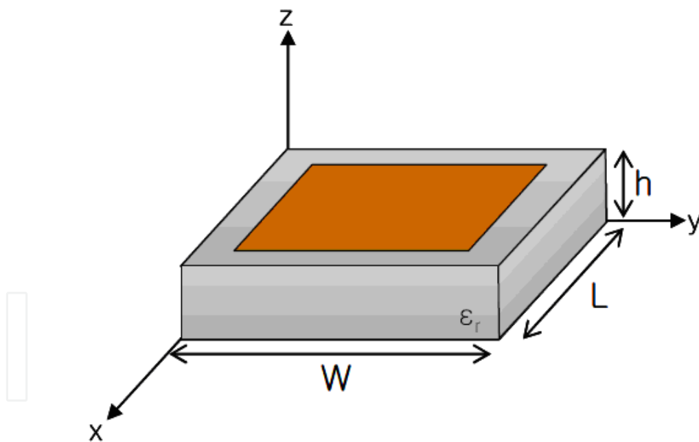
Figure 1. Configuration of the microstrip antenna
