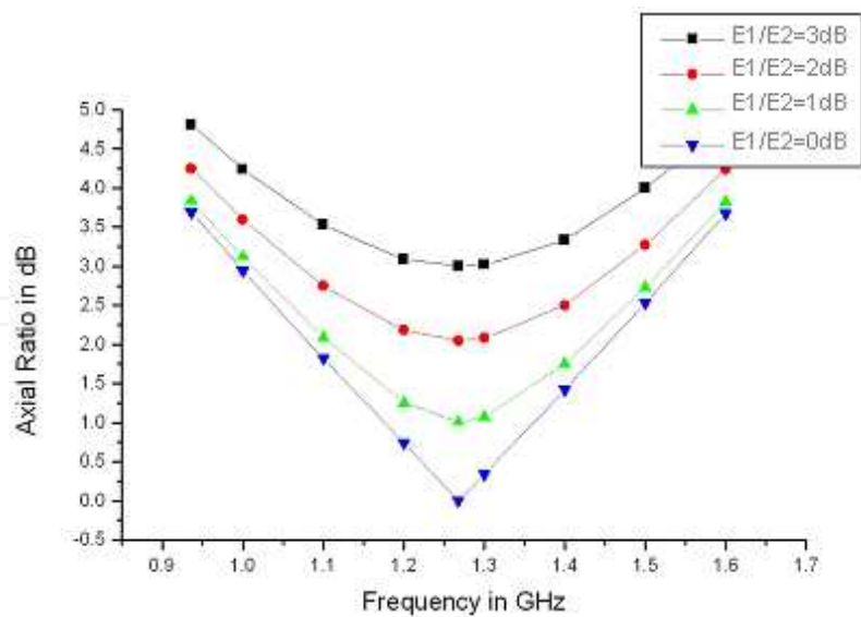
Figure 9. Axial ratio bandwidth of different amplitudes excitation of the two feeds
