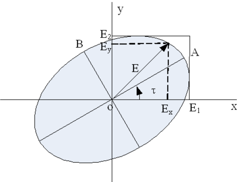
Figure 6. Polarization ellipse
