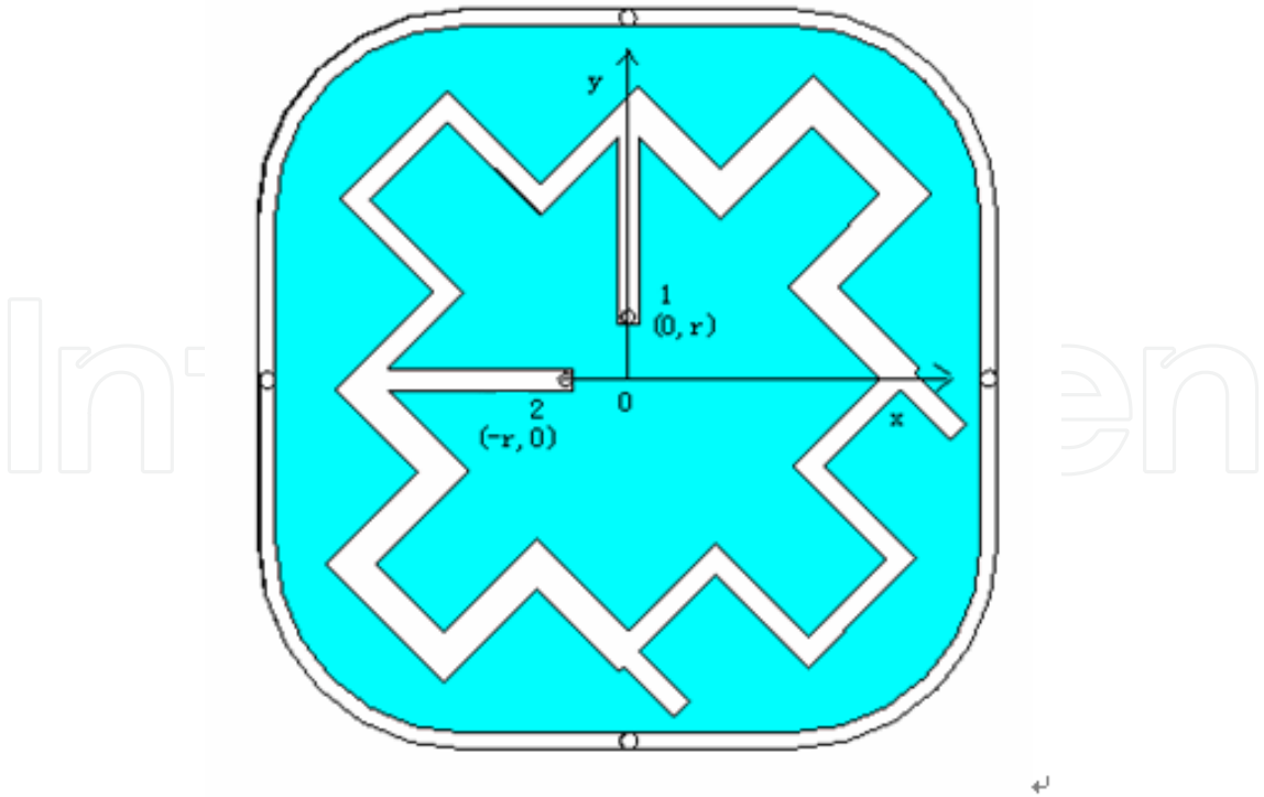
Figure 13. Feed network
