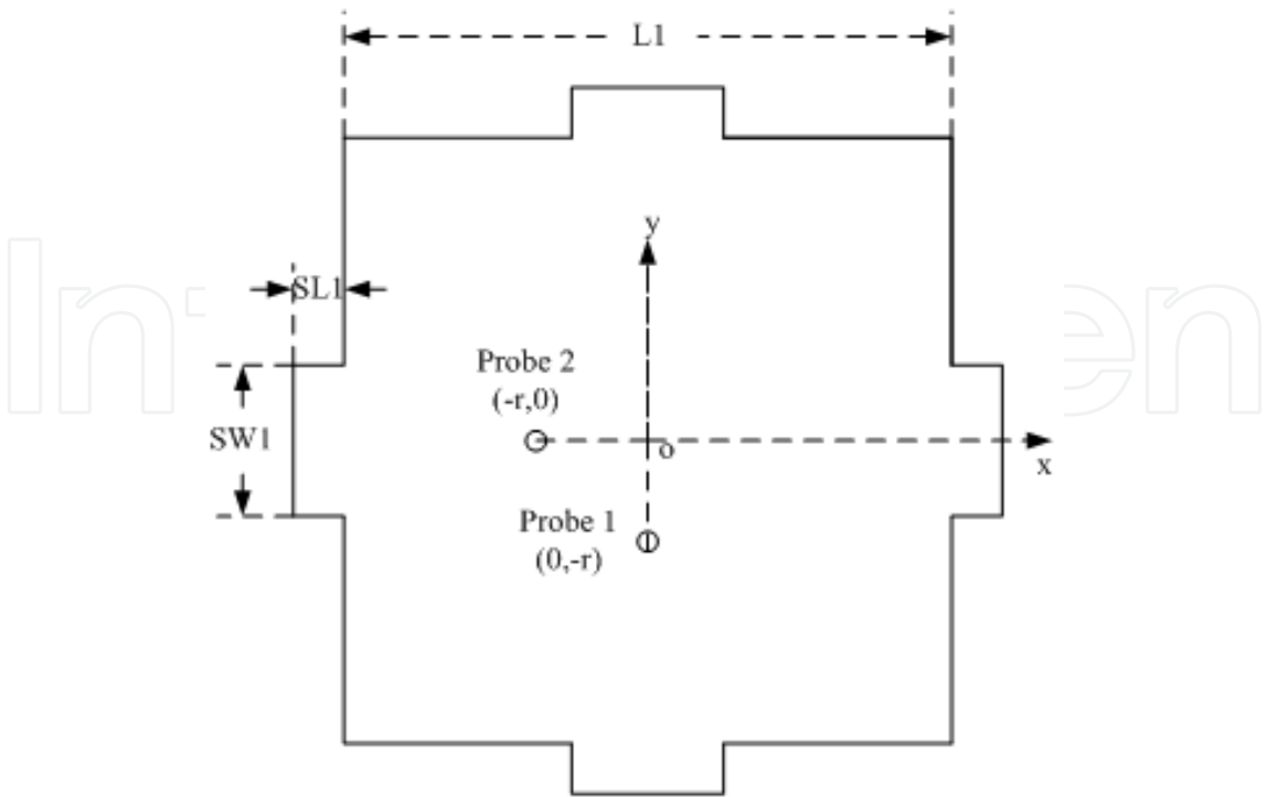
Figure 12. Patch shape
