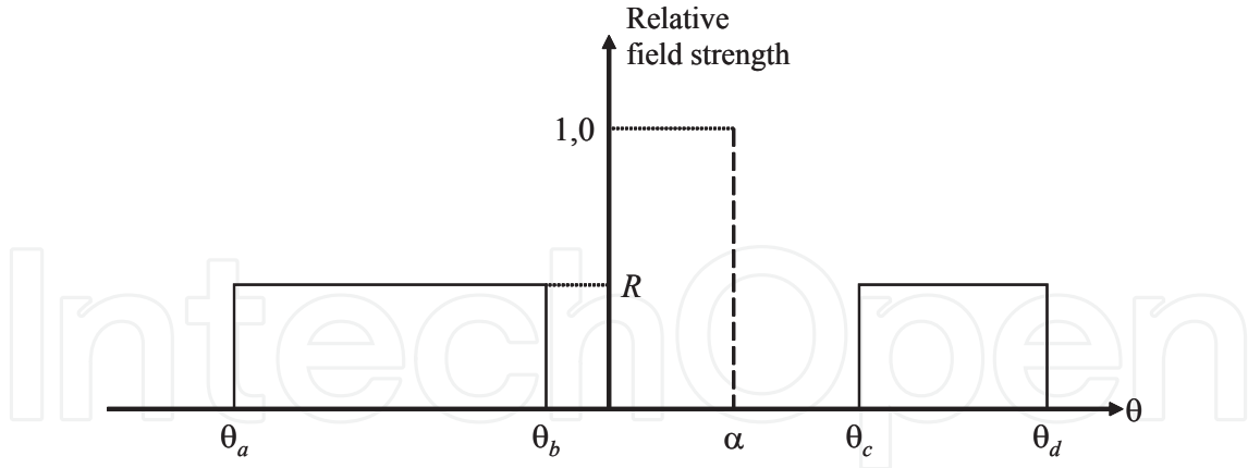
Figure 6. Typical specification of a radiation pattern in a given plane
