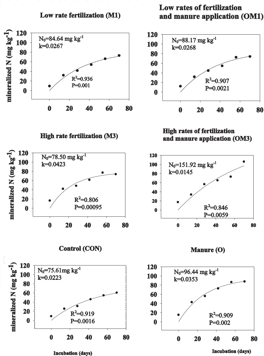
Figure 4. Fitting curves of nitrogen mineralization in fertilization experiment in Uman, Ukraine, as described with the first order kinetic model: N_{min} = N_0(1 - e^{-kt}) , where N_{min} is the mineralized N at time t , N_0 is the potentially mineralizable N (PMN), k is the mineralization rate constant.
