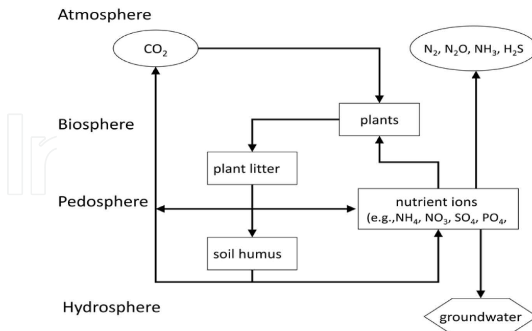
Figure 1. Conceptual model of soil organic matter decomposition (modified from [106])
