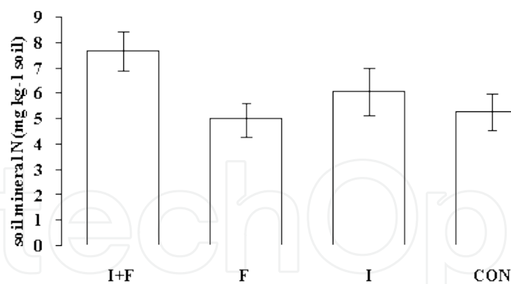
Figure 5. Soil mineral nitrogen in irrigation experiment, Kherson
