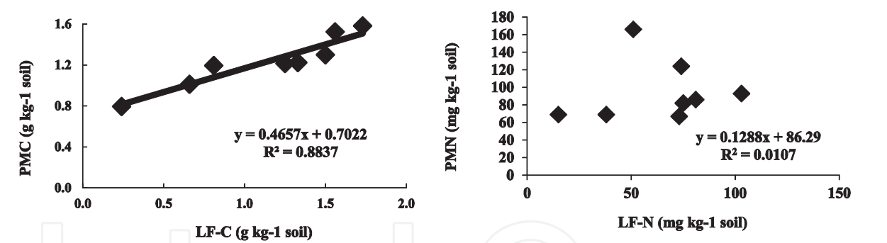
Figure 9. Correlation of potential mineralizable C and N ) with "light" fraction C (LF-C) and N (LF-N)
