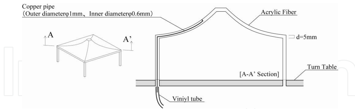
Figure 12. Details of the experimental model
