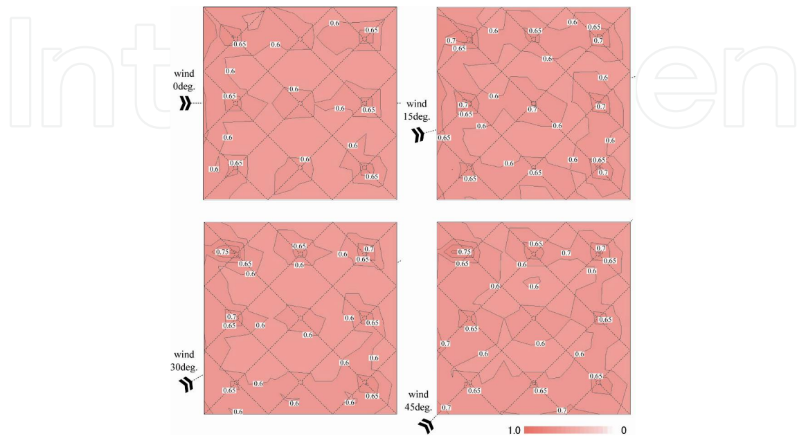
Figure 23. Fluctuating wind pressure coefficient which were obtained from wind tunnel tests on enclosed type of the multi-bay mode
