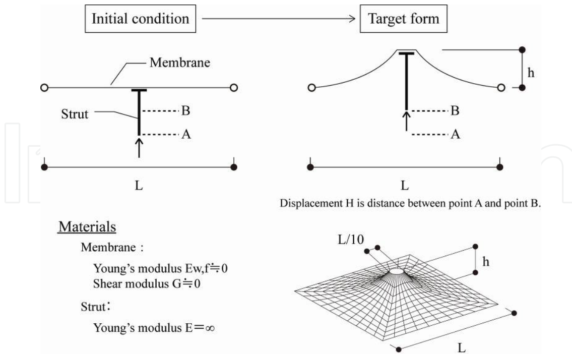
Figure 3. Form finding method on the horn-shaped membrane structure
