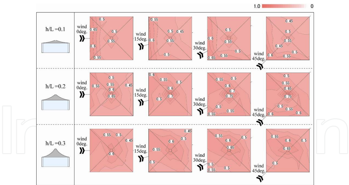
Figure 15. Fluctuating wind pressure coefficient which was obtained from wind tunnel tests on enclosed type of the stand-alone mode
