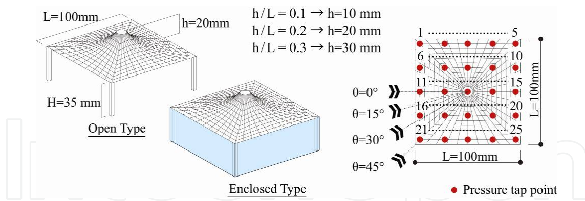
Figure 10. Experimental models and measuring points on the stand-alone models; two types model was prepared, namely “Open type” and “Enclosed type”
