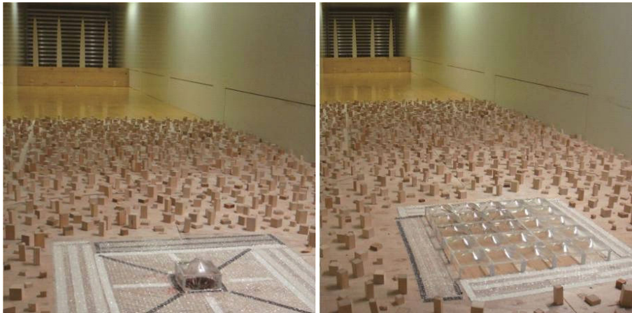
Figure 8. Photos of wind tunnel test
