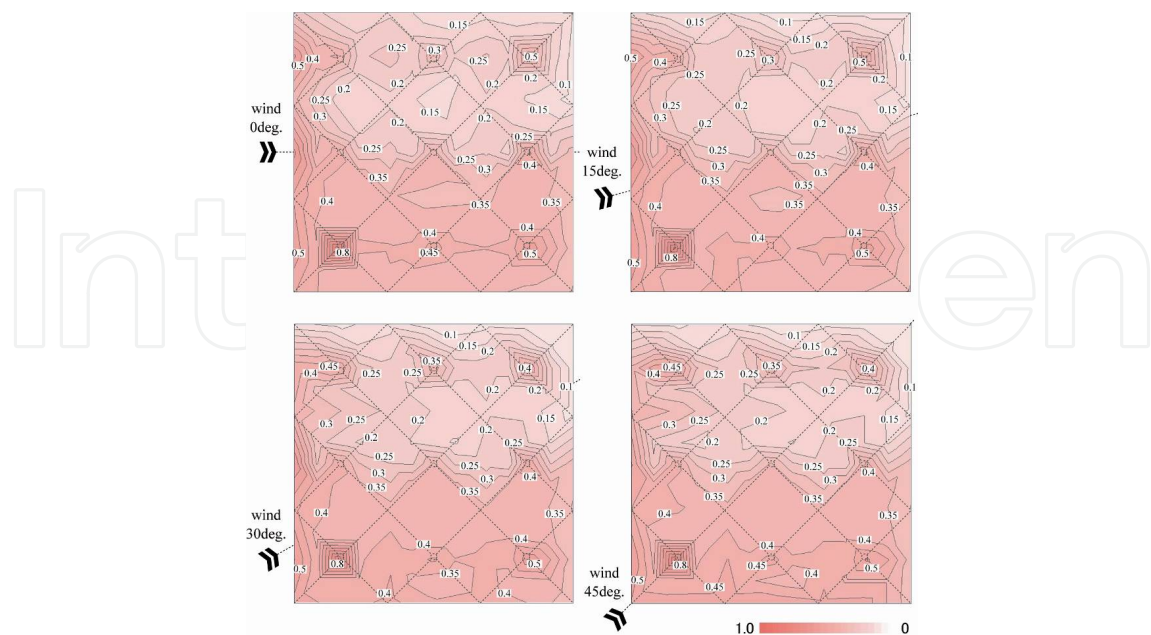
Figure 24. Fluctuating wind pressure coefficient which were obtained from wind tunnel tests on open type of the multi-bay mode
