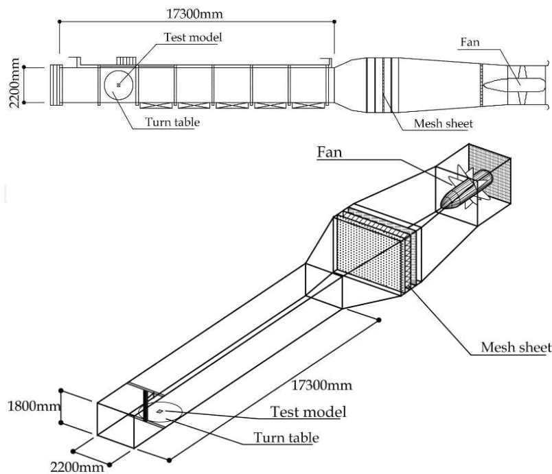
Figure 5. Sketch of Eiffel wind tunnel used
