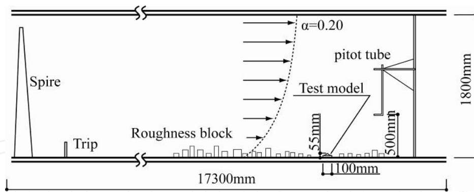
Figure 6. Cross-section diagram of wind tunnel facilities
