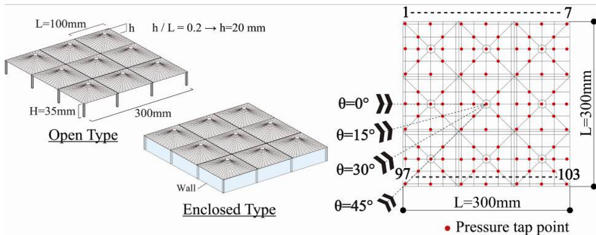
Figure 19. Experimental models and measuring points on the multi-bay models
