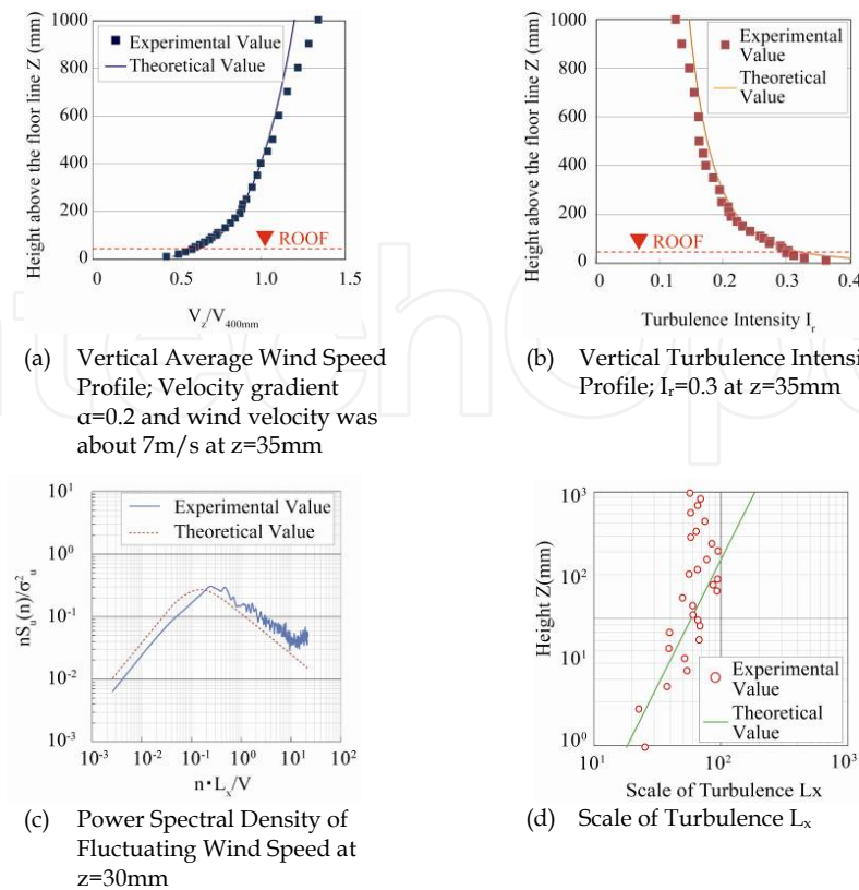
Figure 9. Wind flow conditions in the wind tunnel test
