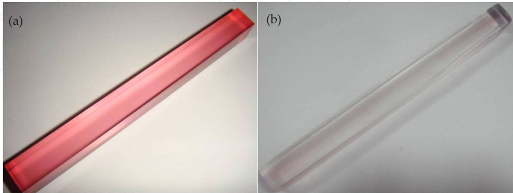
Figure 4. (a) Ti^{3+} :sapphire single crystal, (b) Ti^{4+} :sapphire (annealing 1600°C for 24h from Ti^{3+} :sapphire).
