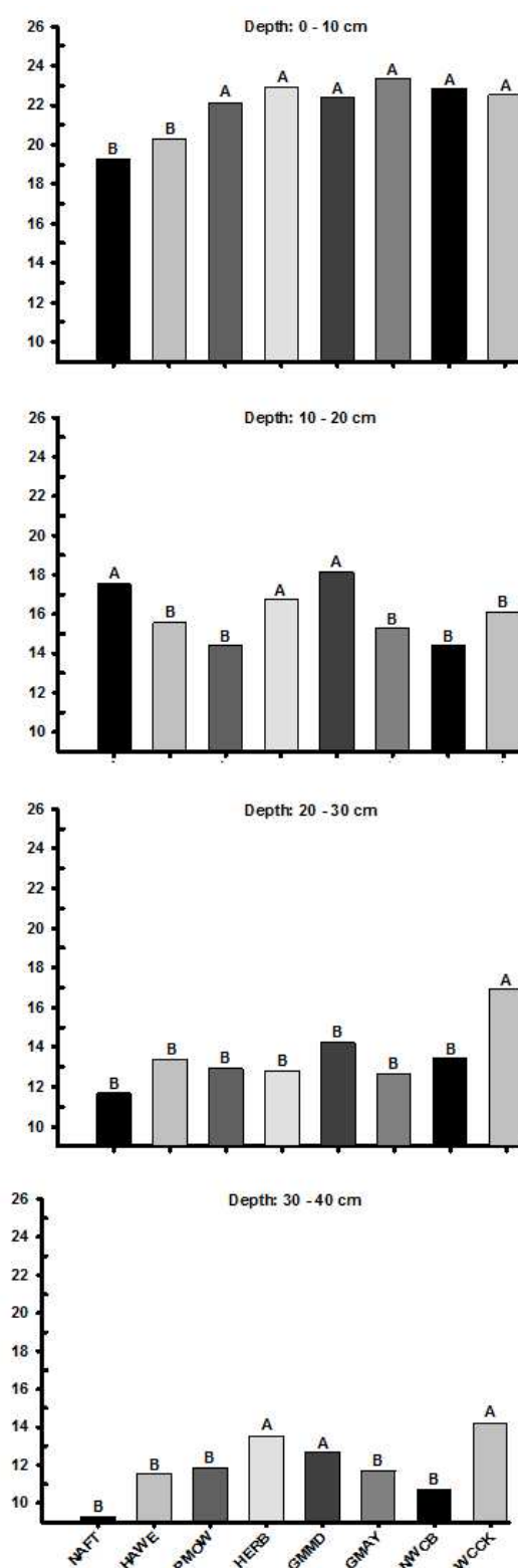
Figure 2. Total soil organic carbon stocks for a Dystroferic Red Latosol at four depths, under natural forest and coffee plantation. NATF: native forest; HWE: hand weeding; HERB: pre plus post-emergence herbicides; PMOW: portable mechanical mower; GMMD: dwarf mucuna ( Mucuna deeringiana ); GMAY: peanut horse ( Arachis hypogaea ); NWCB: no-weed control between coffee rows; WCCK: weed check.
