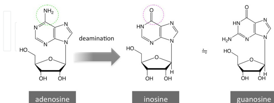
Figure 3. Adenosine deamination by ADARs. ADARs convert adenosines to inosines of double-stranded RNA by catalyzing a hydrolytic deamination at C6 of the adenine base. This modification is called RNA editing, more specifically, A-I editing. Inosine is recognized as guanosine at translation, and this editing produces codon change. Also, it creates alternative splice sites. These both lead to different proteins in the target substrate. Recently a lot of non-coding RNA has also been found to be substrates of ADARs.
