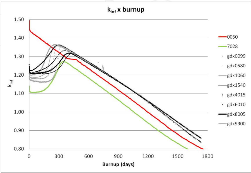
Figure 7. Infinite neutron multiplication factor as a function of burnup – 2.0% Gd 2 O 3 , 6.0% U-235, changing Gd-155 and Gd-157 enrichments.
