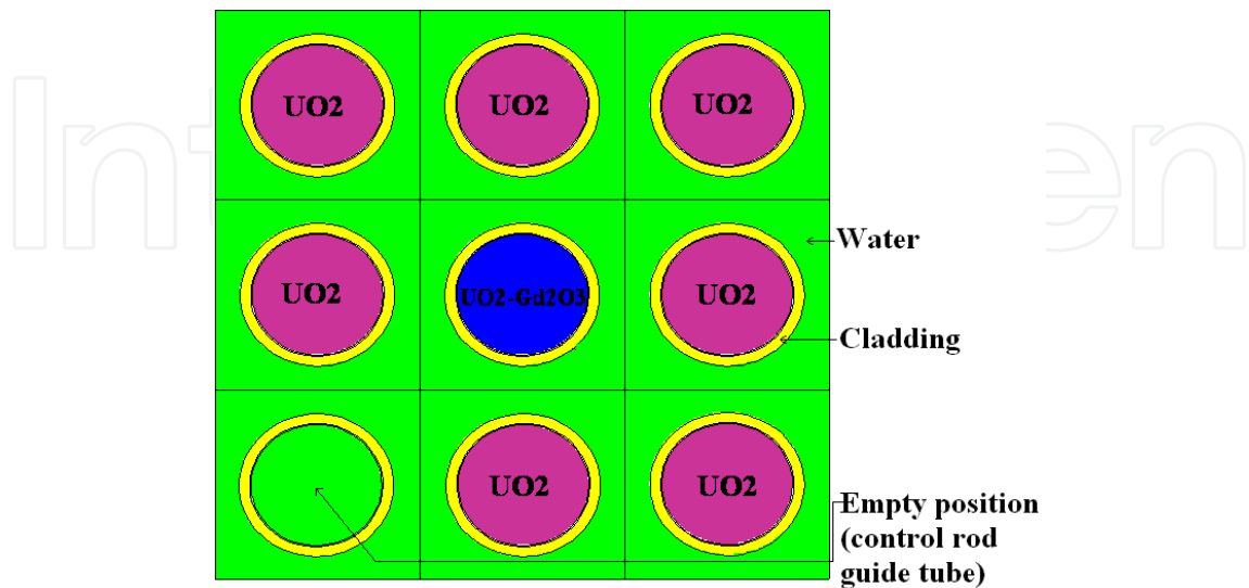
Figure 1. Infinite fuel pin cells 3x3 lattice.
