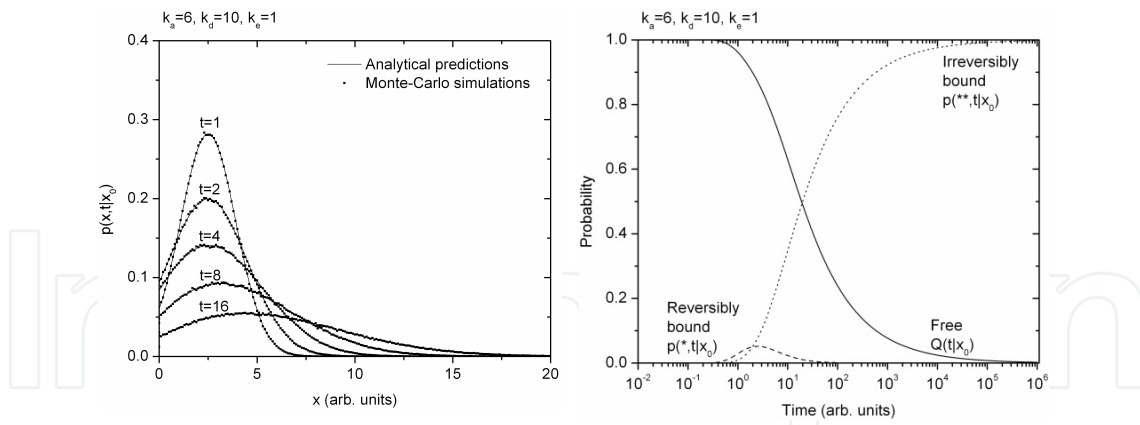
Figure 10. Left) Probability distribution of a particle near a partially absorbing and reflecting boundary with back reaction for x_0=2.5 , k_a=6 , k_d=10 , k_e=1 and D=1 ( \alpha=1 , \beta=2 and \gamma=3 ) at t=1, 2, 4, 8 and 16 time units. The lines are the analytical predictions p(x, t | x_0) . The dots are given by the simulation of 1,000,000 particle histories either with one or multiple time steps. (Right) Probability of a particle in these conditions to be free, reversibly bound or irreversibly bound as a function of time.
