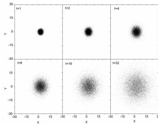
Figure 5. Positions of 1,000,000 particles initially located at x_0=2.5 , y_0=0 at t=1, 2, 4, 8, 16 and 32 time units. The positions are obtained by sampling the Green's function as described in Algorithm 4 or 5.
