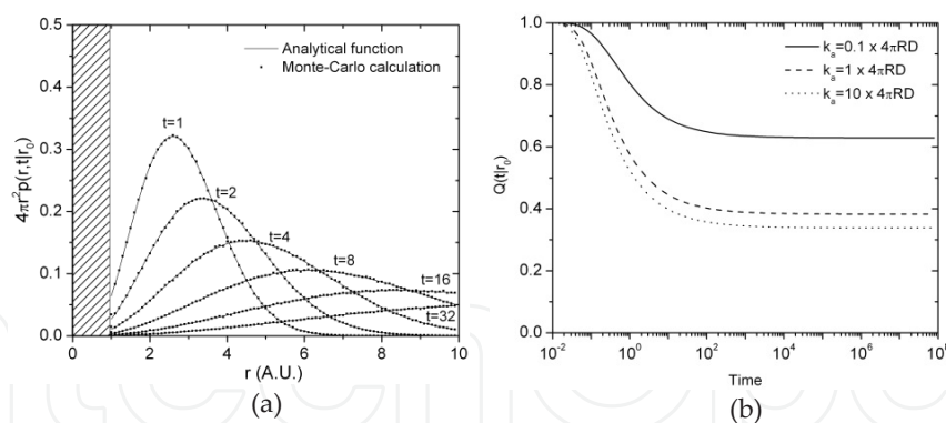
Figure 11. a) Green's function 4\pi r^2 p(r, t | r_0) for D=1 , R=1 , r_0=1.5 and \alpha=-2 at t=1, 2, 4, 8, 16 and 32 . Analytical functions: (—); Result of sampling: (■). b) Survival probability Q(t | r_0) as function of time for D=1 , R=1 , r_0=1.5 and k_a=0.1 \times 4\pi RD (—), 4\pi RD (---) and 10 \times 4\pi RD (·).
