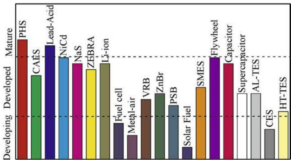
Figure 17. Technical maturity of EES systems [69]
