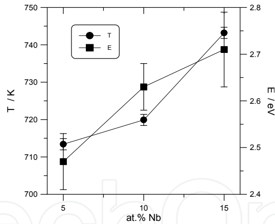
Figure 18. Apparent activation energy and peak temperature of the crystallization process against Nb content for alloys A, B and C milled for 160 h [58].
