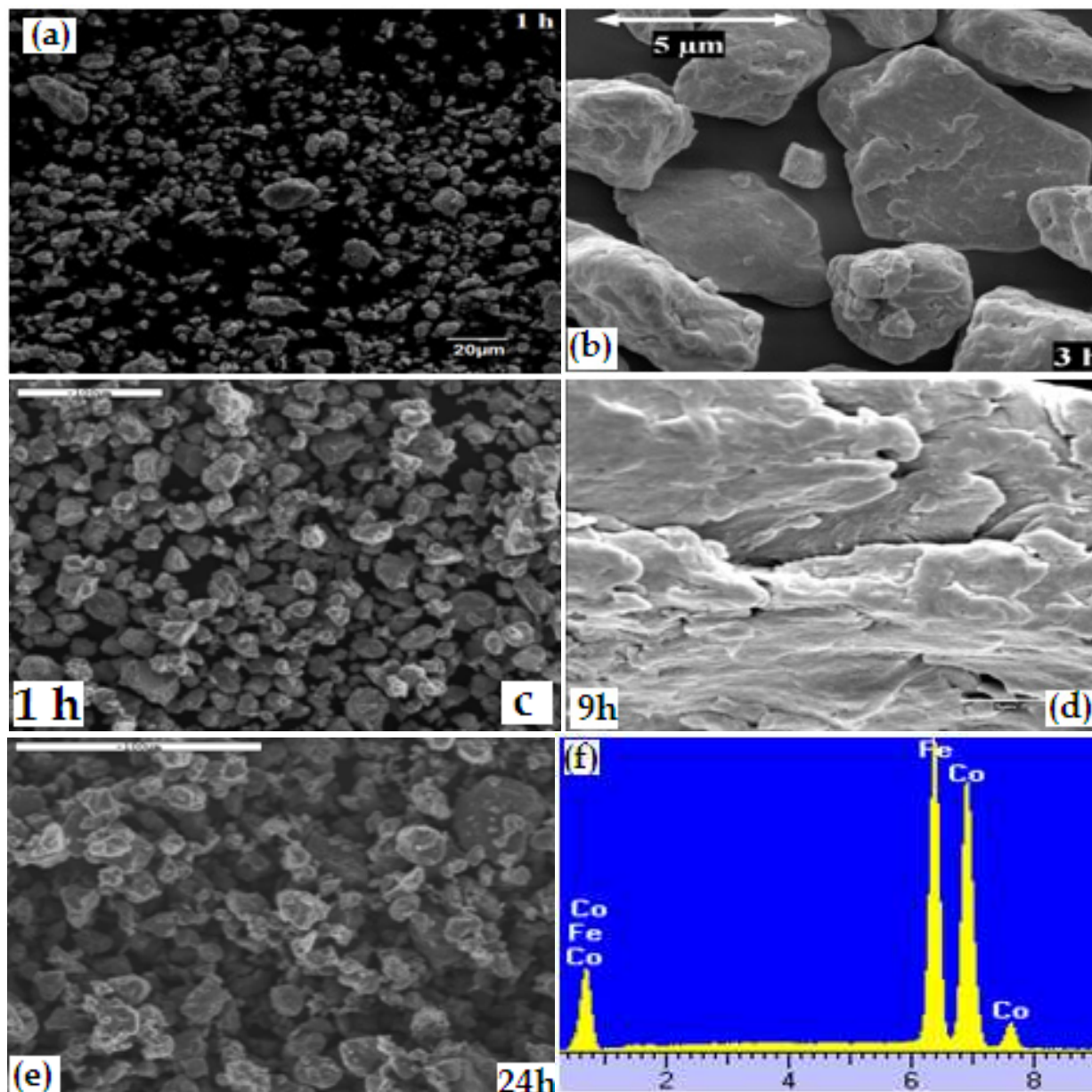
Figure 2. Morphologies of powder particles of the ball-milled \text{Fe}_{75}\text{Si}_{15}\text{B}_{10} (a), \text{Ni}_{20}\text{Co}_{80} (b), \text{Fe}_{57}\text{Cr}_{31}\text{Co}_{12} (c and d), and \text{Fe}_{50}\text{Co}_{50} powders (e) with the corresponding EDX analysis (f).
