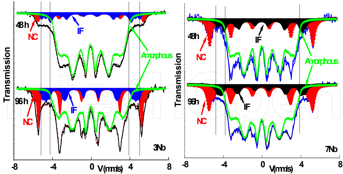
Figure 9. Room temperature Mössbauer spectra of 3Nb and 7Nb powders milled for 48 and 96 h [55].
