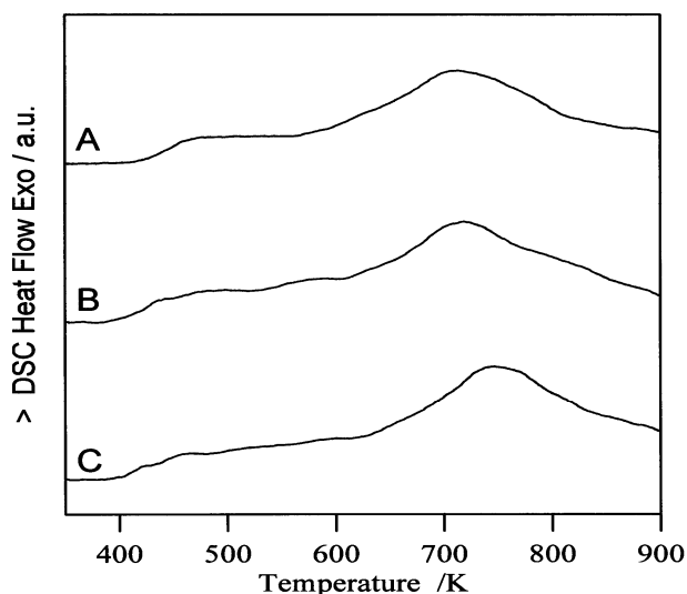
Figure 15. DSC scans at a heating rate of 10 K.min -1 of the ball-milled A, B and C powders for 160 h [58].
