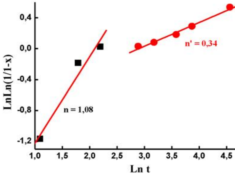
Figure 23. Johnson-Mehl-Avrami plot of the ball-milled \text{Fe}_{57}\text{Co}_{21}\text{Nb}_7\text{B}_{15} versus milling time [27, 66].
