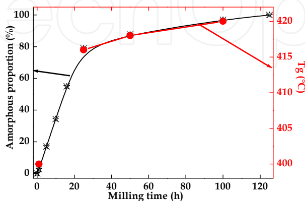
Figure 16. Variation of the glass transition temperature and the amorphous phase proportion of the (Fe 50 Co 50 ) 62 Nb 8 B 30 powders as a function of milling time.
