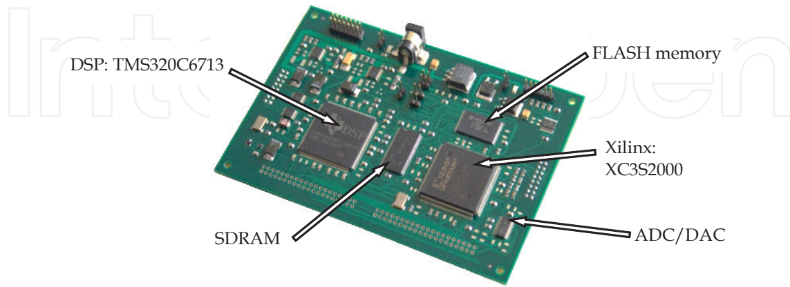
Figure 18. Protoplate board of dynamic reconfigurable pipeline DWPT processor
