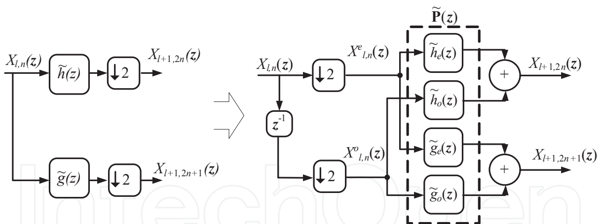
Figure 5. The transition to the polyphase implementation of analysis filter bank
