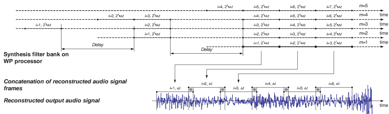
Figure 27. The output signal synthesis in DWPT processor
