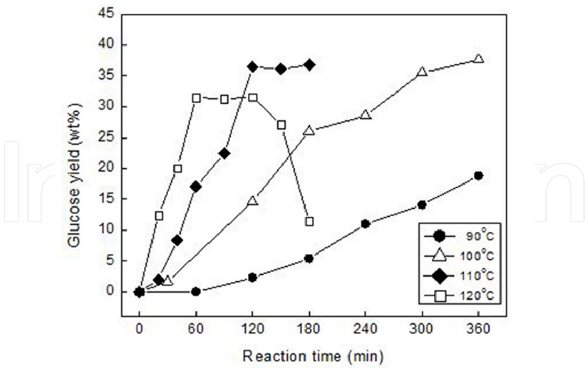
Figure 15. Changes in glucose yield from cellulose treated in [C2mim][Cl] with 0.5 wt% sulfuric acid at various reaction temperatures
