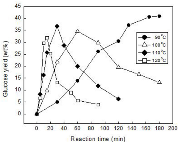
Figure 14. Changes in glucose yield from cellulose treated in [C2mim][Cl] with 1.5wt% of sulfuric acid at various reaction temperatures.
