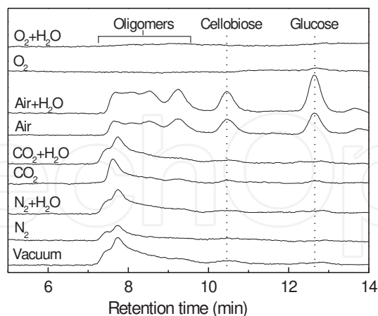
Figure 13. High performance liquid chromatograms of the solubilized compounds in [C2mim][Cl] obtained by 24 h treatment under various reaction atmospheres
