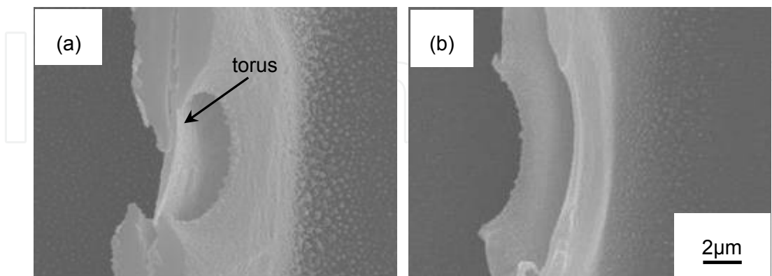
Figure 11. SEM images of bordered pit-pair in earlywood in tangential sections after treatment by [C2mim][Cl] at 120 °C for 0 h (a) and 48 h (b)
