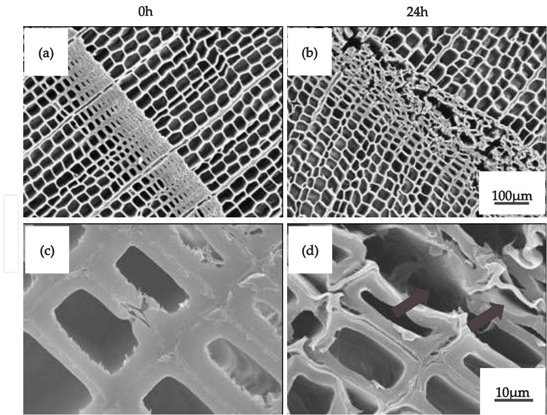
Figure 9. SEM images of transverse sections treated with [C2mim][Cl] at 120°C for 24 h. (a,c) 0 h treatment, (b,d) 24 h treatment.
