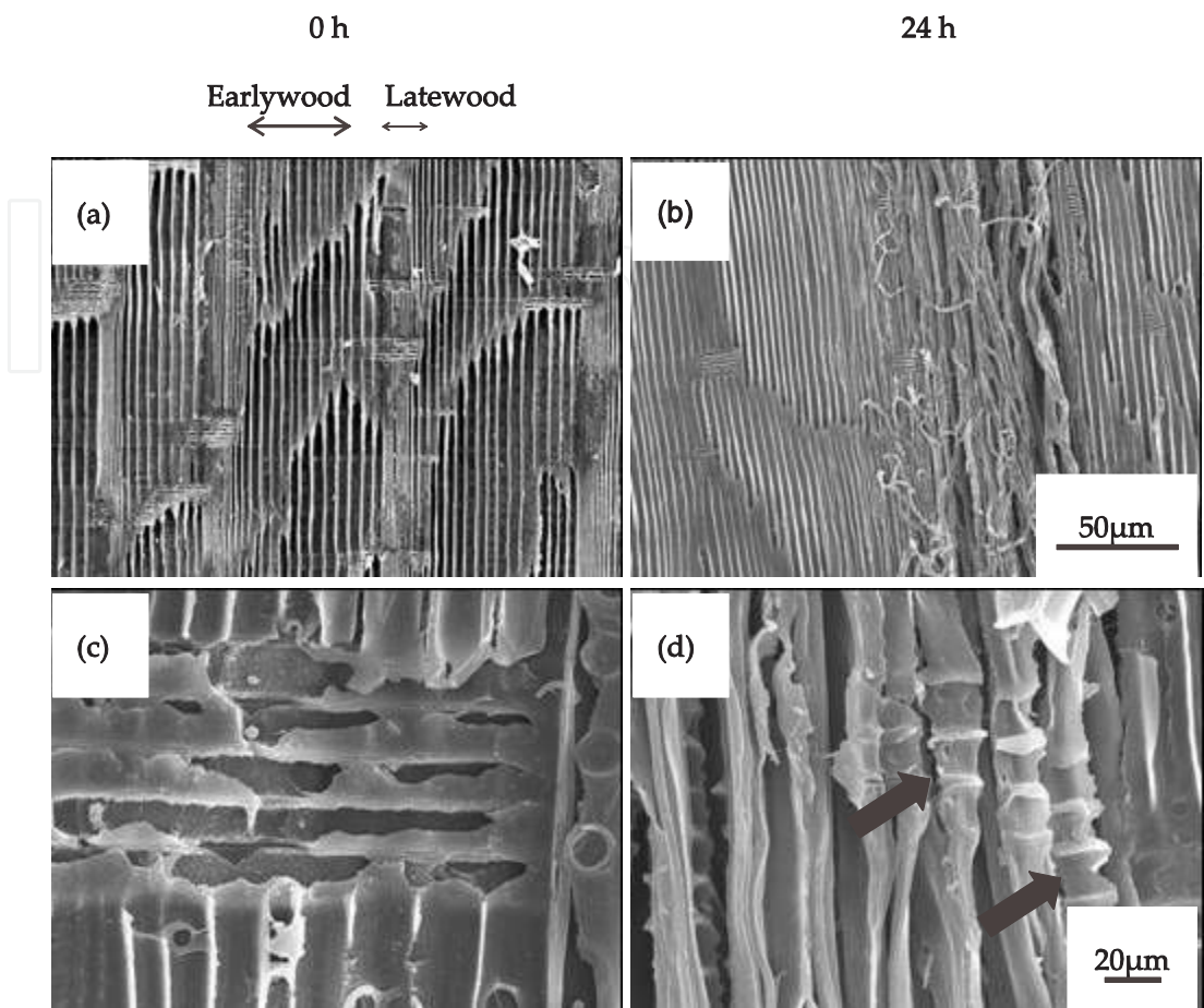
Figure 10. SEM images of radial sections after treatment with [C2mim][Cl] at 120 °C for 24 h. (a,c) 0 h treatment, (b,d) 24 h treatment.
