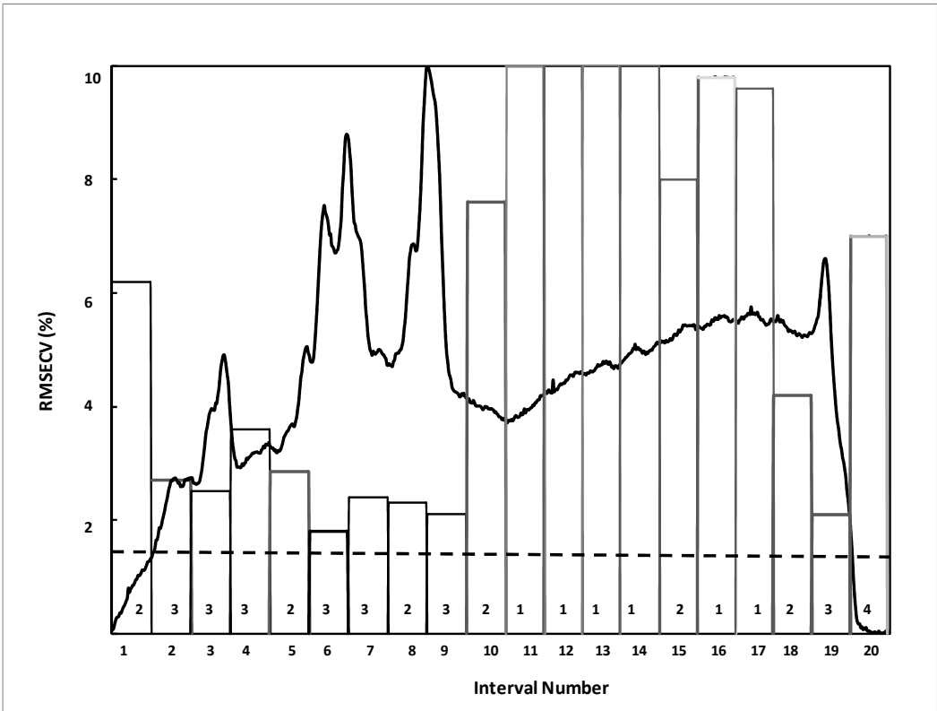
Figure 9. RMSECV values for PLS models obtained for the 20 different intervals (bars) used in iPLS models. The horizontal dotted line represents the RMSECV value for the PLS model with all variables. Numbers inside the rectangles are the optimal number of latent variables.
