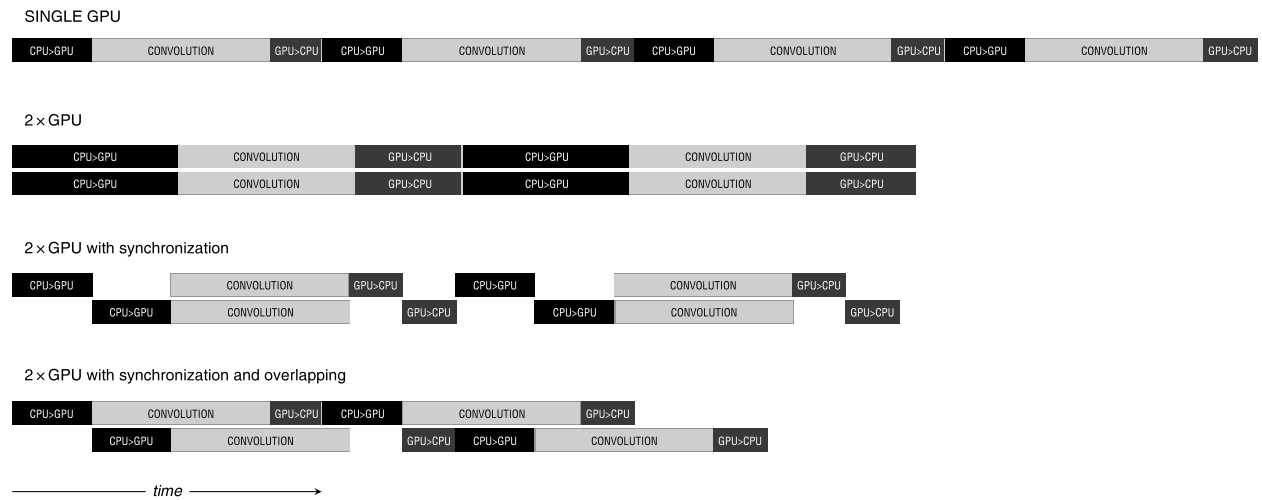
Figure 8. A model timeline of the algorithm workflow [21]. The dark boxes denote data transfers between CPU and GPU while the light boxes represent convolution computations. The first row shows the single-GPU implementation. The second row depicts parallel usage of two GPUs. The data transfers are performed concurrently but through a common bus, therefore they last twice longer. For the third row, the data transfers are synchronized so that only one transfer is made at a time. In the last row, the data transfers are overlapped with the convolution execution.
