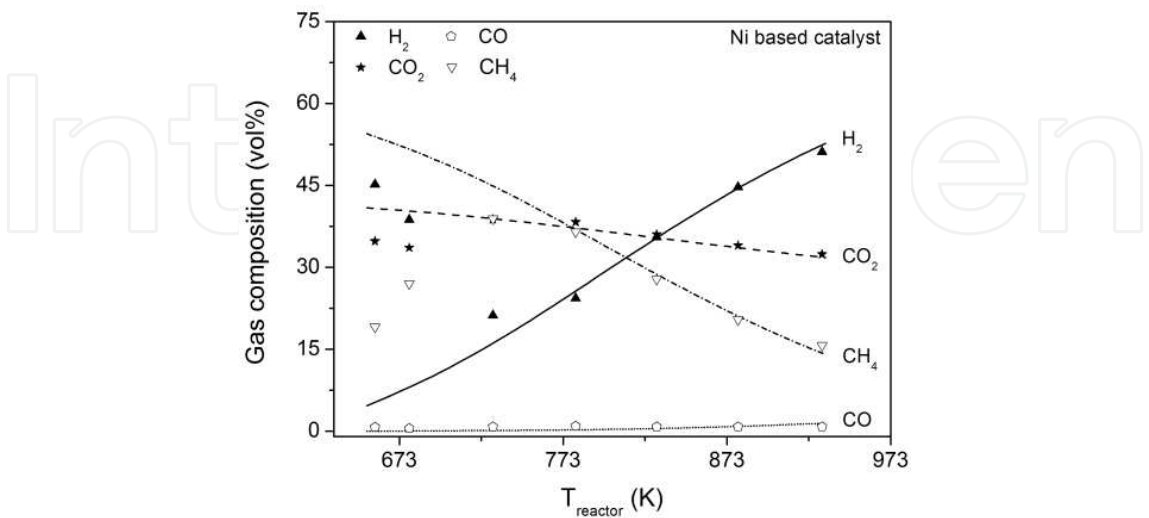
Figure 8. Gas concentration as a function of the temperature for a Ni based catalyst. P = 25.5 - 27.0 MPa, [glycerol] = 10 wt%. The curves represent equilibrium compositions, the symbols are experimental points [29].
