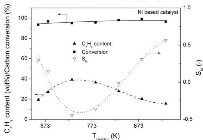
Figure 9. Performance indicators. P = 25.5 - 27.0 MPa, [\text{glycerol}] = 10 wt%, \phi_{\text{gly}} = \pm 100 g/h. The lines are trend lines and for illustrative purposes only.
