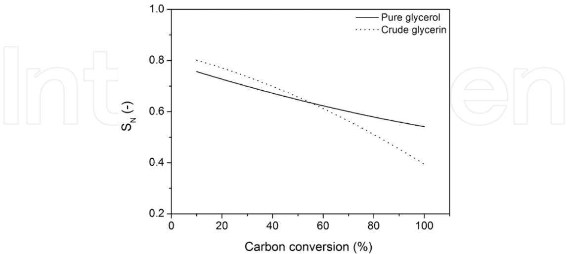
Figure 7. S_N for pure glycerol and crude glycerin as a function of the carbon conversion.
