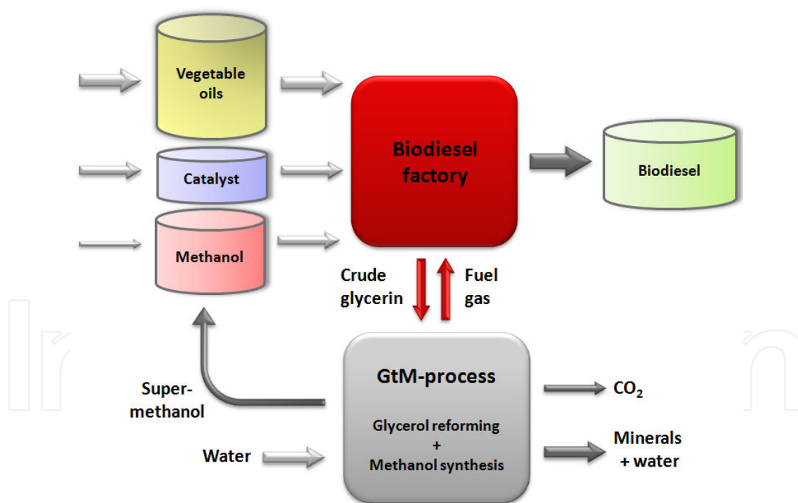
Figure 2. Outline of the Supermethanol concept. The glycerol-to-methanol (GtM-) process is the process under investigation in the Supermethanol project.
