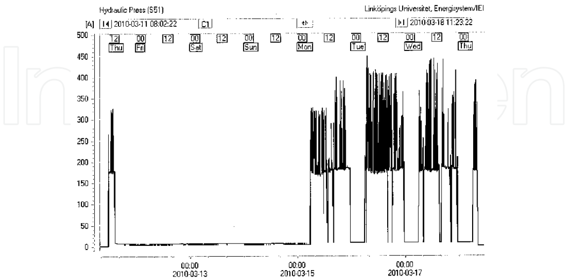
Figure 9. The current used by a hydraulic press during one week.
