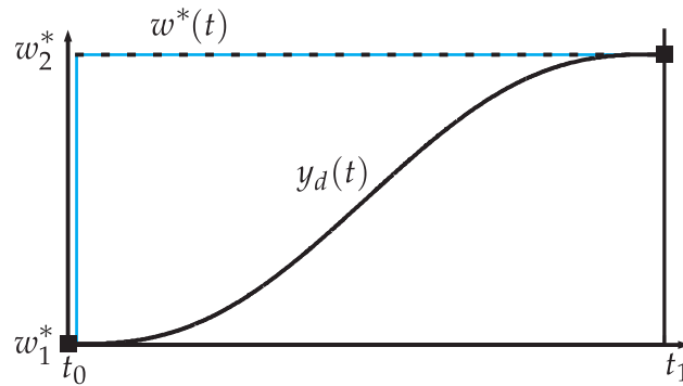
Figure 7. Illustration of a general input signal \Delta w^*(t) and the resulting output signal y_d(t) of the trajectory generator \Sigma_{traj}^* within a fixed transition time T = t_1 - t_0 .
