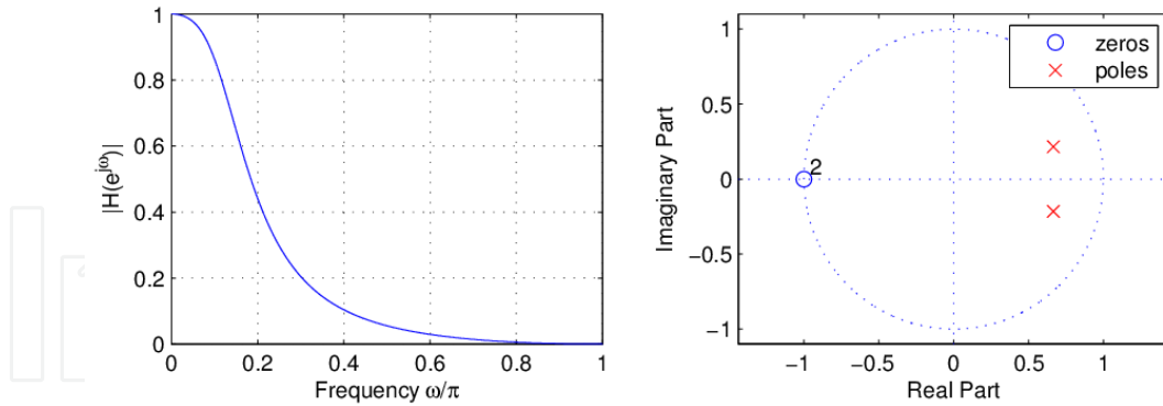
Figure 2. Frequency responses and zero-pole configurations of H(z) .
