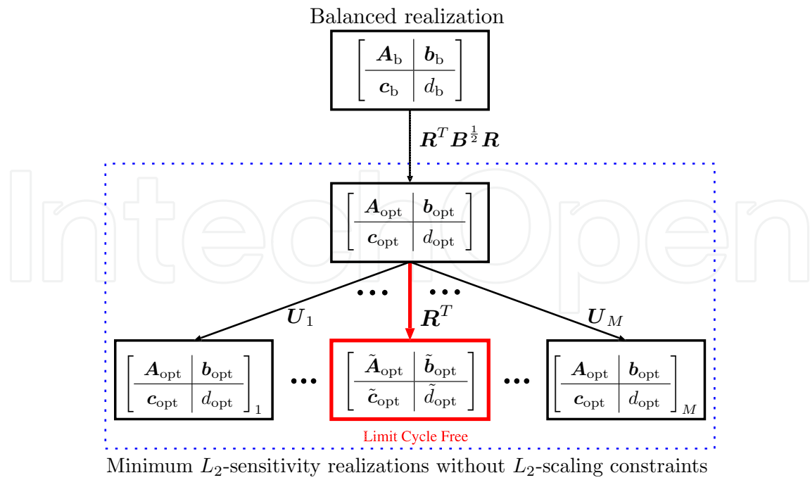
Figure 6. Synthesis of the minimum L_2 -sensitivity realization which does not generate limit cycles.
