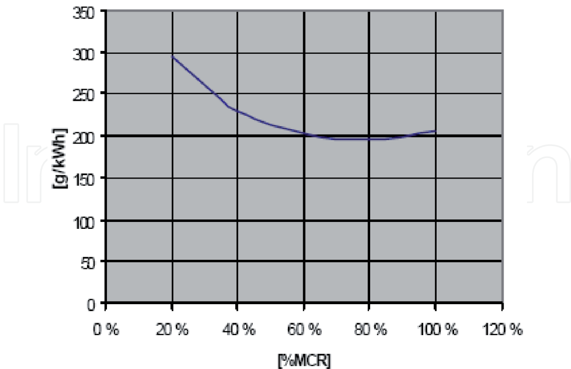
Figure 10. Diagram of the specific consumption of diesel engine as a function of maximum continuous power [31, 32].
