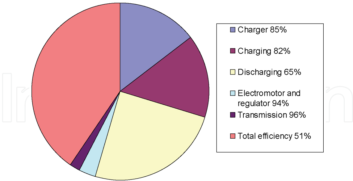
Figure 18. Diagram of losses and efficiency of electric vehicles.
