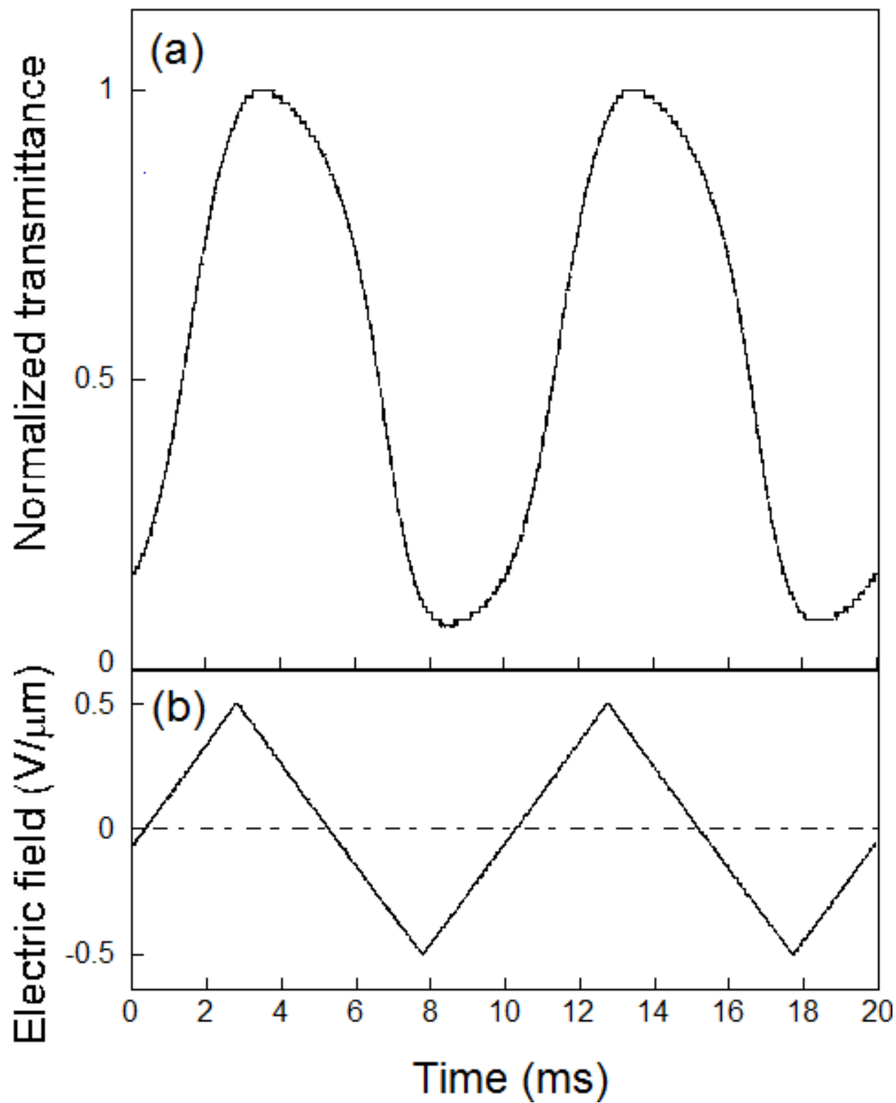
Figure 24. Switching behaviour of SCE8 mixed with 2 wt% CDH and 0.1 wt% TNF under a 100 Hz, \pm 0.5 Vm/\mu m triangular wave electric field. (a) Transmittance of light through the FLC under a polarizing microscope. (b) Magnitude of the applied electric field.
