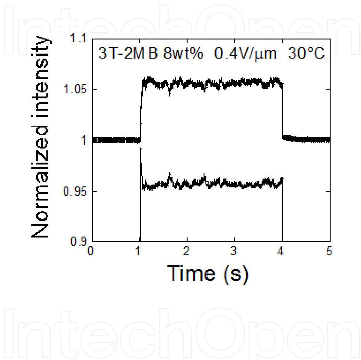
Figure 17. Examples of the results of two-beam coupling experiments for mixtures of the base LC, 3T-2MB and TNF measured at 30 °C.
