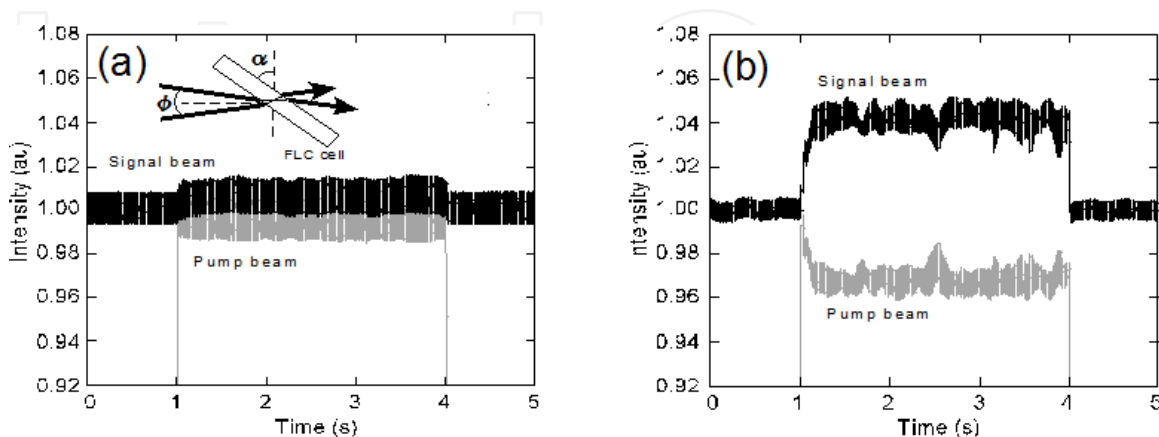
Figure 33. Asymmetric energy exchange with a square waveform of 2.0 \text{ V}_{p-p}\mu\text{m}^{-1} , 100 Hz (a) without bias, and (b) with a bias of 0.5 \text{ V}\mu\text{m}^{-1} . The intersection angle \phi was 20^\circ and the sample angle \alpha was 50^\circ .
