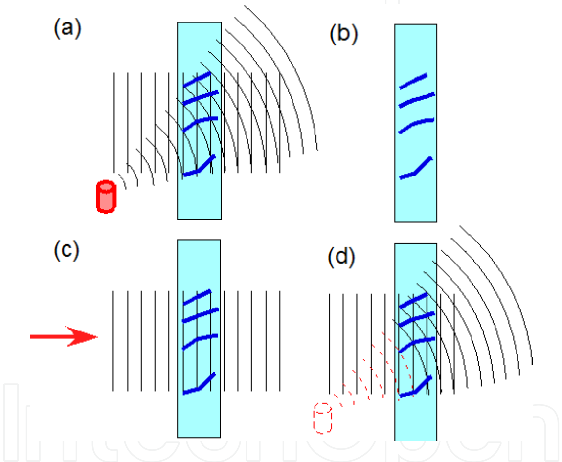
Figure 1. Hologram recording and image reconstruction. (a) A light reflected from an object is interfered with by a reference light in a photo-sensitive material, such as a photopolymer. (b) The interference fringe is recorded in a photosensitive material (hologram). (c) A readout beam is irradiated by the hologram. (d) The readout beam is diffracted by the hologram and the object image is reconstructed.
