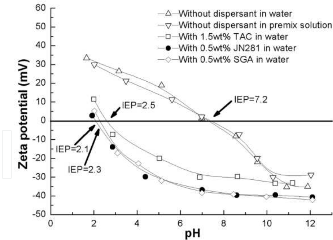
Figure 2. Effect of dispersants on the zeta potentials of the PZT suspensions at different pH values.
