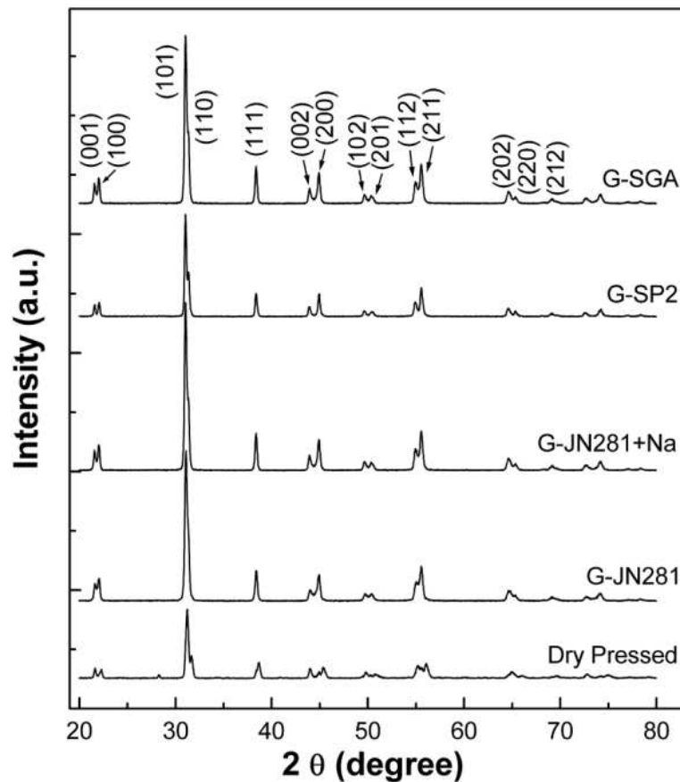
Figure 9. XRD patterns of different PZT samples.
