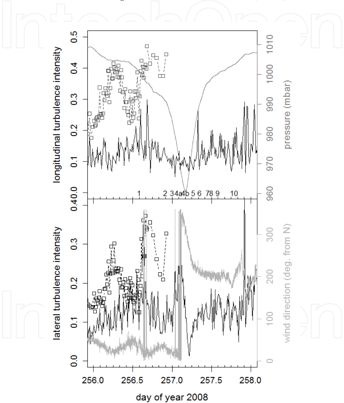
Figure 7. Turbulence intensities as measured by the sonic and top level cup anemometers as compared to storm passage characteristics of pressure (top panel) and wind direction (bottom panel). Lateral turbulence intensity of the 034B sensor depicted in the bottom panel is assessed from the 1-min wind direction fluctuation (right axis) and plotted as 10 \times \sigma_{wd} / 360 (left axis). Note the surprise lull under northwesterly wind directions towards the end of the eyewall passage.
