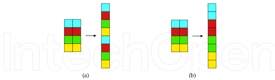
Figure 2. Different types of supervector composition; (a) composition with simple concatenating, (b) composition with retaining the structure of the basic vector
