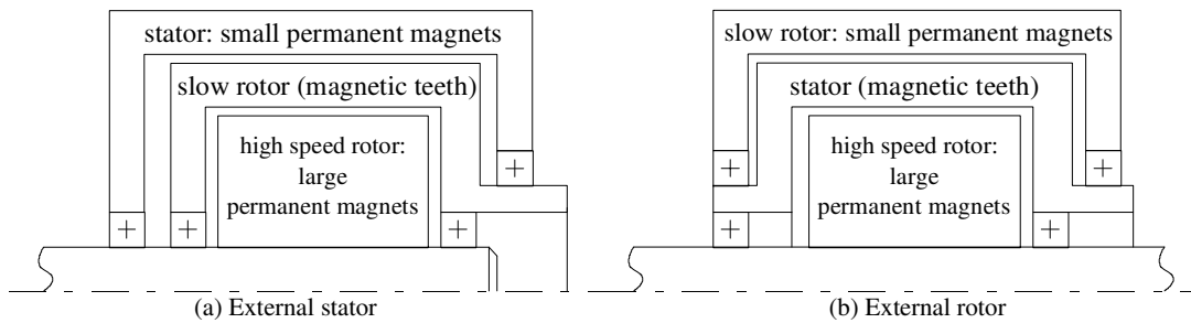
Figure 12. Arrangement of the bearings in cylindrical structure
