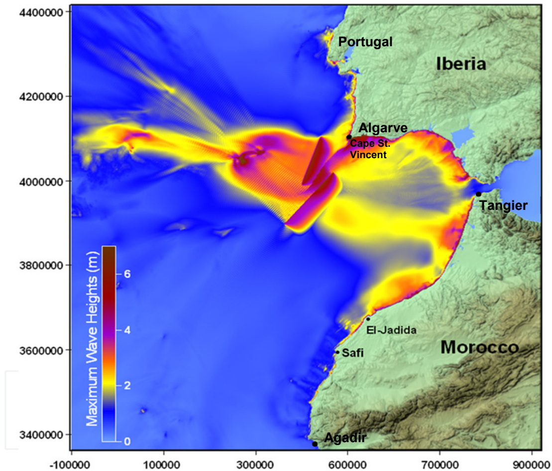
Figure 5. Maximum wave heights distribution in the Gulf of Cadiz region due to the occurrence of HSF+MPF earthquake scenario of Mw8.6.
